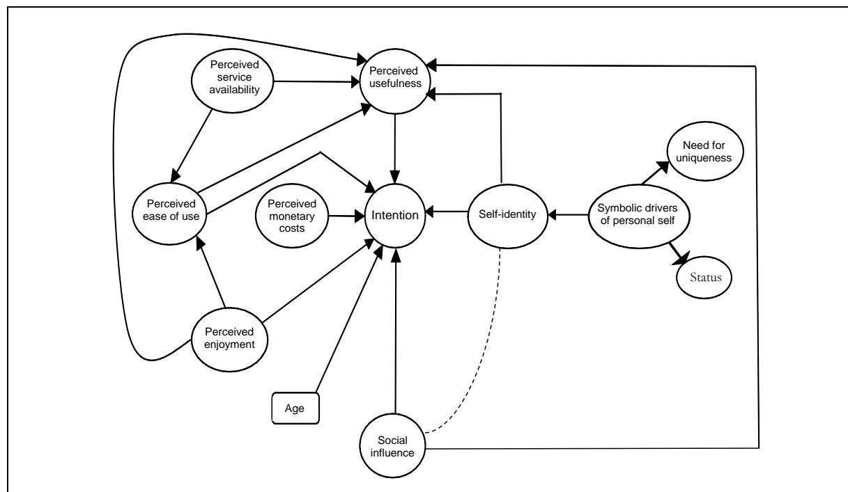
Figure 2. Re-specification of Hong and Tam (2006) model
