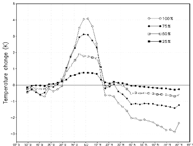
Figure 3. Latitudinal pattern of temperature change with different deforestation fractions.
