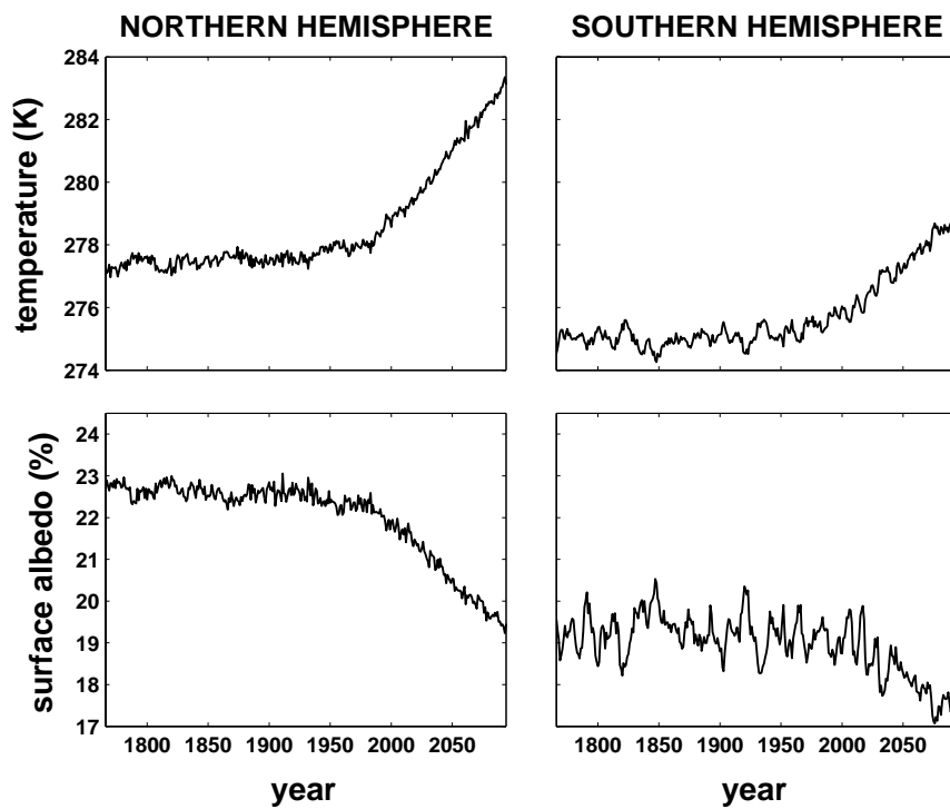
Figure 9: Annual-mean time series from the scenario run of SAT and surface albedo averaged over NH and SH polar caps bounded by 30° latitude.
