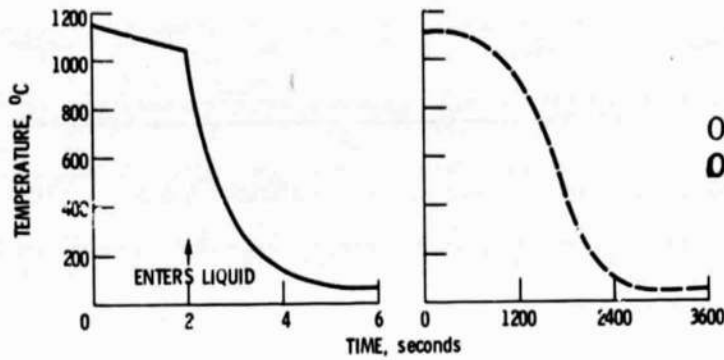
(a) FAST COOLING (WATER QUENCH). (b) SLOW COOLING.
