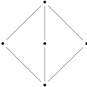
FIGURE 1. The 1-3-1 lattice
