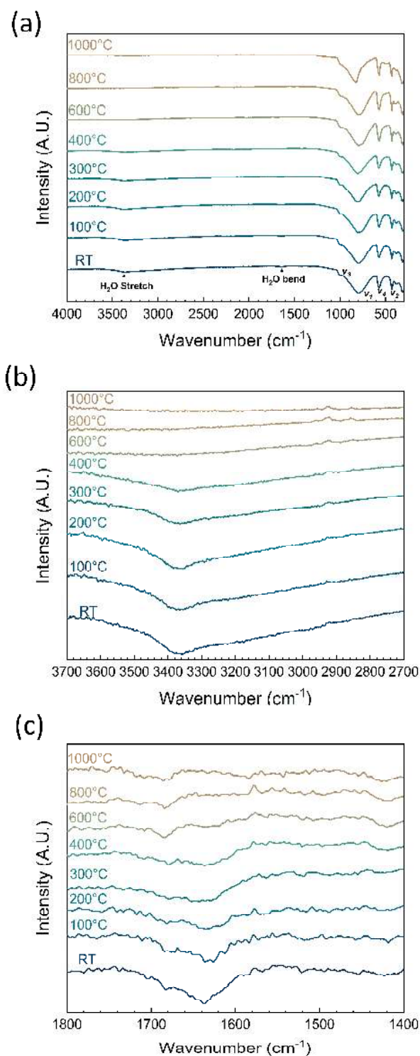
Figure 10. FTIR performed on pristine and calcinated stettindite for temperatures ranging from room temperature to 1000°C in the regions (a) 4000-300 \text{cm}^{-1} , (b) 3700-2700 \text{cm}^{-1} and (c) 1800-1400 \text{cm}^{-1} . Arrows and labels indicate what the various vibrational bands are attributed. \nu_1 , \nu_2 , \nu_3 , \nu_4 are the 4 normal internal modes of vibration.
