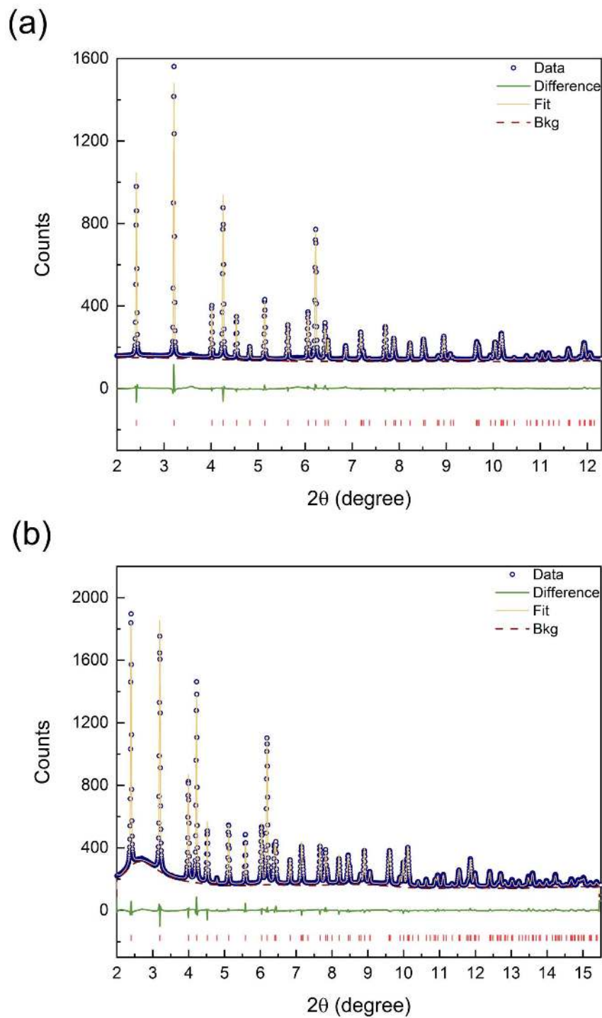
Figure 2. Fitted synchrotron XRD patterns of (a) stetindite at 27°C and (b) coffinite at 31°C. Data are shown as open blue circles , and the solid yellow curve is the best fit to the data. The solid green curve represents the difference between the observed and calculated profiles. The red tick marks above the x-axis indicate the positions of diffraction maxima.
