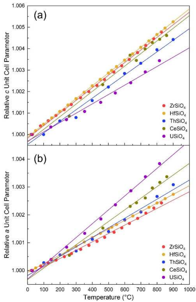
Figure 14. Comparison of the thermal expansion obtained for unit-cell parameters (a) c and (b) a for several anhydrous MSiO_4 compounds (data from this study for M = Ce, U and data from the literatures for M = Zr, Hf, Th ). 89,111,112
