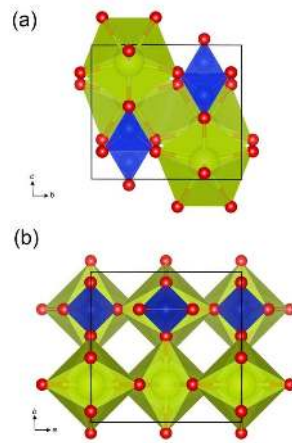
Figure 1. Projections of the structure of stetindite down to various crystallographic axes (prepared using the VESTA 3 software package 132 ). In both a and b the yellow dodecahedra are the \text{CeO}_8 , the blue tetrahedra are the \text{SiO}_4 , and the red spheres are oxygen. (a) representation of the structure along [100]. (b) illustration of the structure along [001] showing clearly the channels where water may reside.
