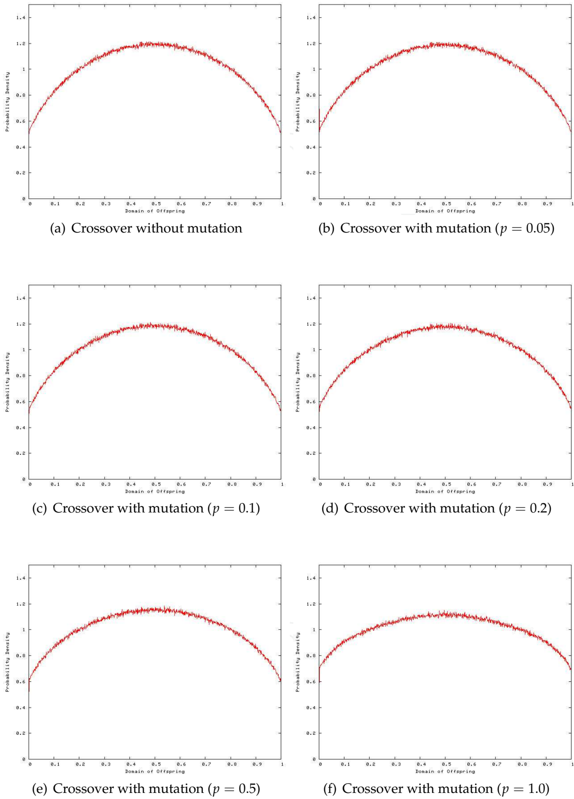
Fig. 10. Bias of extended-box crossover ( \alpha = 0.5 ) with mutation
