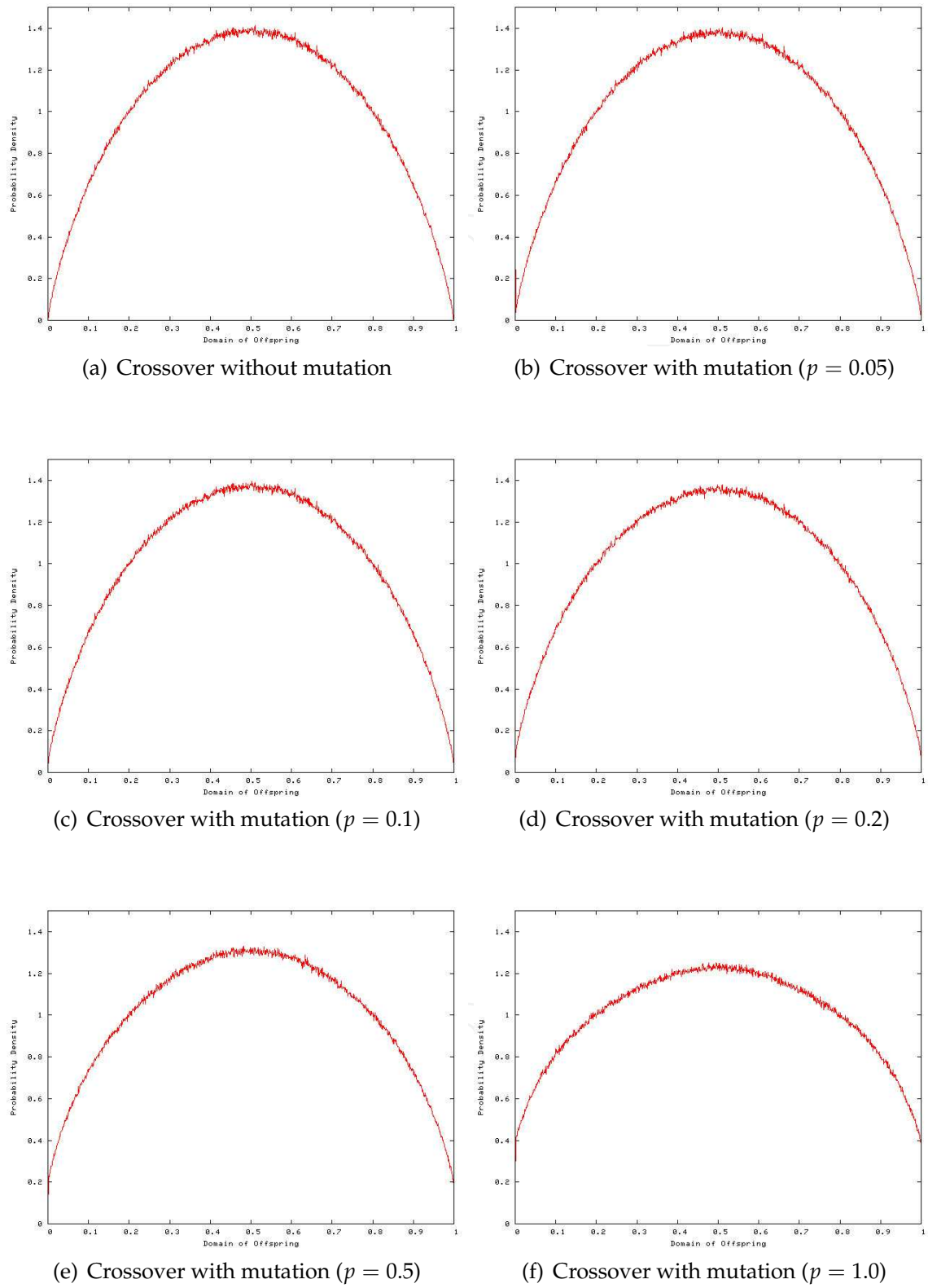
Fig. 11. Bias of line crossover with mutation
