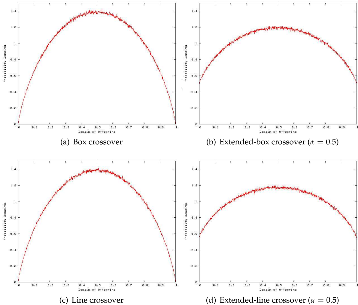
Fig. 8. Crossover bias in one-dimensional bounded real space
