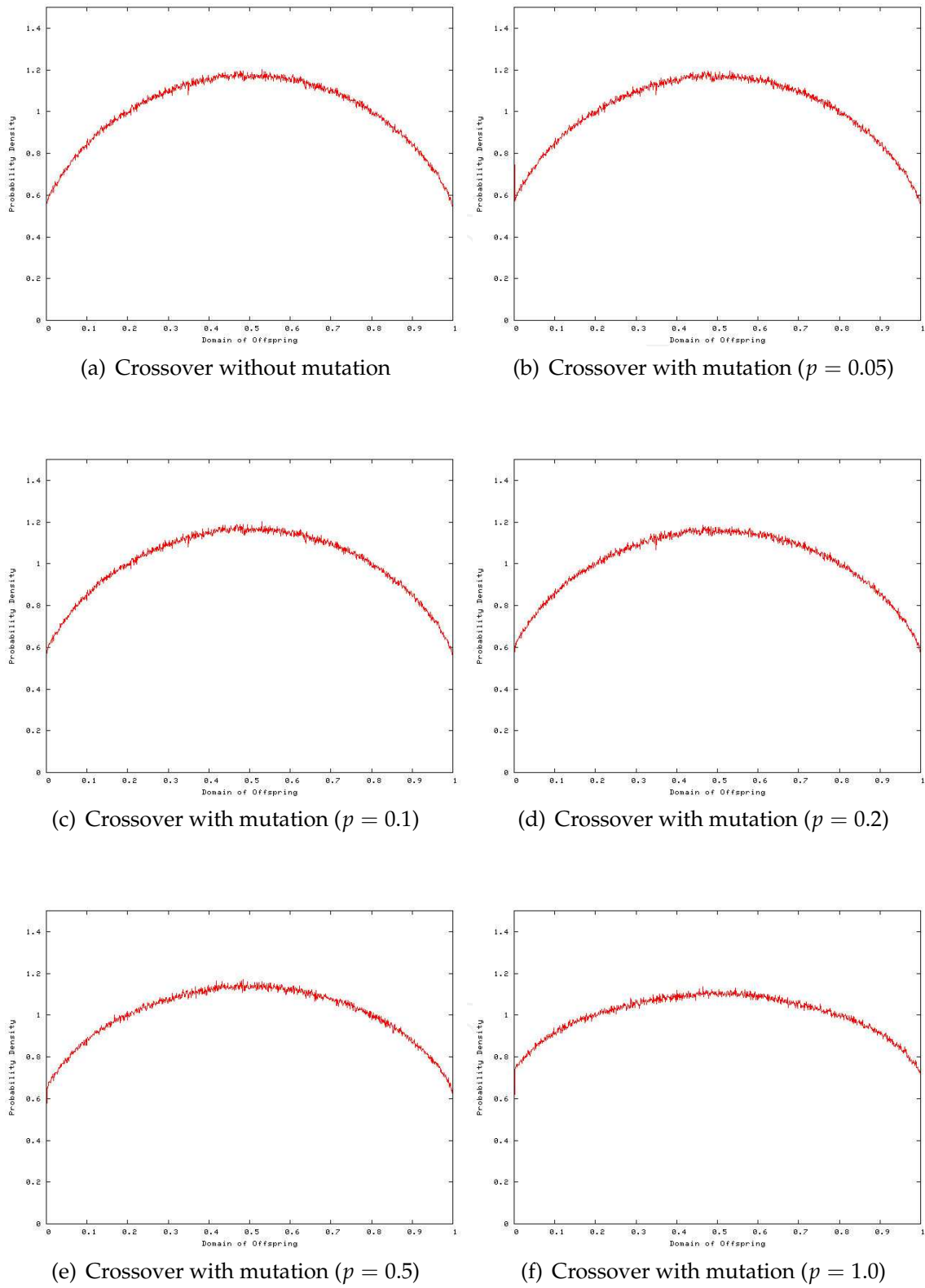
Fig. 12. Bias of extended-line crossover ( \alpha = 0.5 ) with mutation
