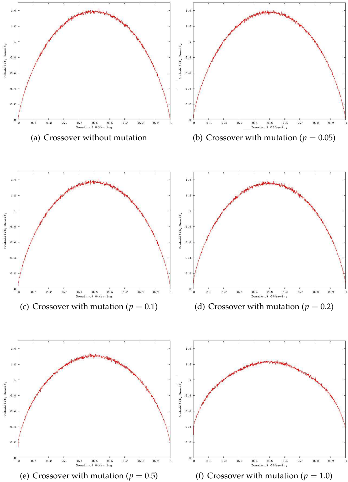
Fig. 9. Bias of box crossover with mutation
