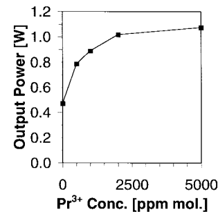
Fig. 9. The influence of lifetime quenching by Pr 3+ co-doping on the calculated output power. The values of the lifetimes of upper and lower laser levels for different Pr 3+ concentrations are taken from [12] and [20] and are reproduced in Table I. The given Pr 3+ concentrations and Er 3+ lifetimes are valid for 40000 ppm mol. Er 3+ concentration, whereas the Er 3+ concentration used for the calculation is 20000 ppm mol.
