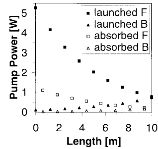
Fig. 2. Launched and absorbed pump power in forward direction ( F ) and after reflection by the mirror at the rear fiber end ( B ) versus fiber length.
