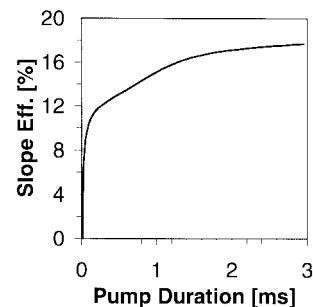
Fig. 6. Temporal evolution of the slope efficiency with respect to launched pump energy under pulsed excitation. Relaxation oscillations are suppressed in this simulation.
