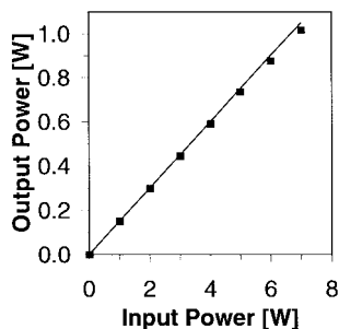
Fig. 5. Calculated input-output curve (squares) of the double-clad diode-pumped erbium 2.7- \mu\text{m} fiber laser. The slope efficiency (solid line) is 15% versus incident pump power and 19% versus launched pump power. The threshold is in the order of a few milliwatts. The small saturation effect of the output power at high pump power is owing to the onset of ESA losses.
