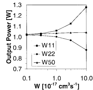
Fig. 8. The influence of upconversion W_{11} from the ^4I_{13/2} lower laser level, upconversion W_{22} from the ^4I_{11/2} upper laser level, and cross relaxation from the ^4S_{3/2} + ^2H_{11/2} levels on the calculated output power.
