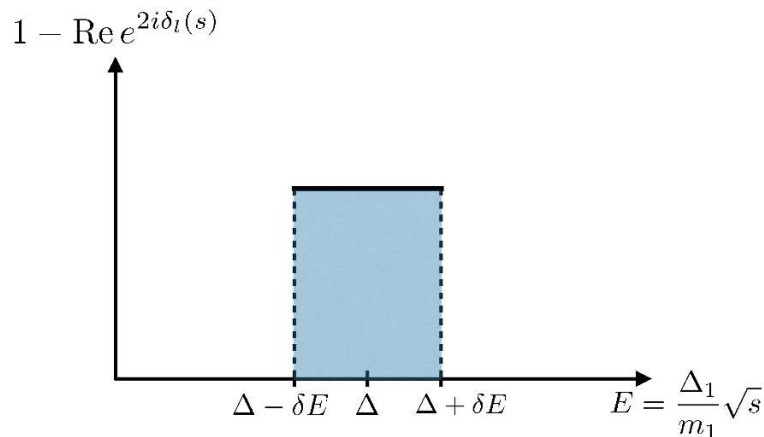
Figure 14. Each operator of dimension \Delta and spin l makes a localized contribution to 1 - \text{Re} e^{2i\delta_l(s)} . The height of the rectangle is given by (C.68). In the flat space limit this contribution becomes proportional to \delta(s - m^2) . The sum over the contribution of all operators produces a smooth function of s .
