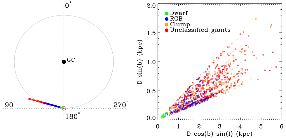
Fig. 1. Location of SAGA targets in the Galaxy. Stars with different seismic classification have different colours, as labelled. Left panel: face-on view in Galactic coordinates, where the distance of each seismic target from the Sun ( D ) is projected along the line of sight D \cos(b) having direction l \approx 74^\circ and Galactic latitude b . The distance between the Galactic Centre (GC) and the location of the Sun ( \odot ) is marked by the solar circle (in gray). Galactic longitudes ( l ) at four different angles are indicated. Right panel: same stars as function of Galactic height Z = D \sin(b) and projected across the l = 90^\circ direction.
