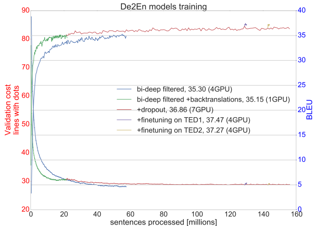
Figure 2: German-to-English models training progress. Plot shows the BLEU (straight lines) and validation error (lines with dots) on tst2015. Colors represent successive training parameters modifications. The number in plot label is the best BLEU score for particular training configuration.
