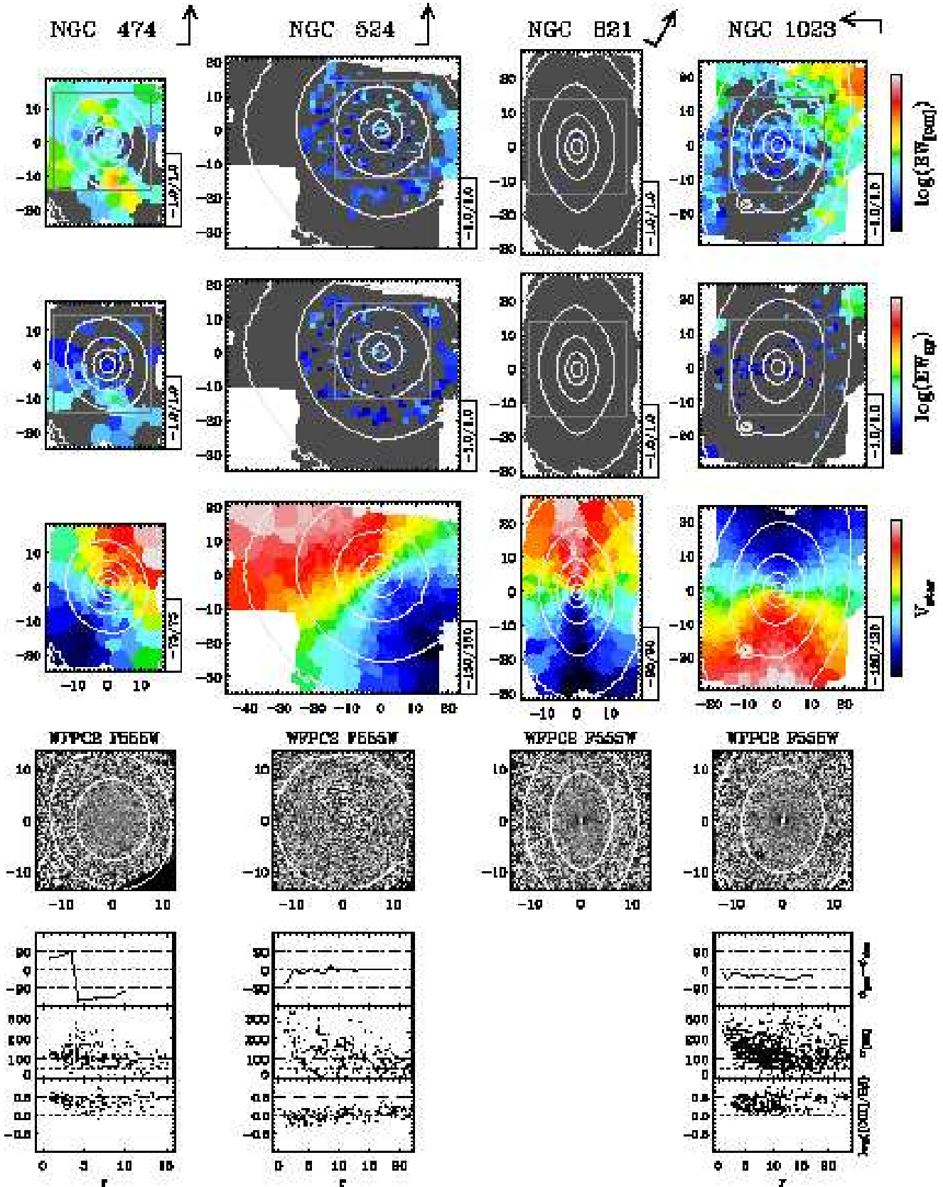
Figure 4b. From top to bottom: i) and ii) equivalent width of the [O\ III]\lambda 5007 and H\beta emission lines, in \text{\AA} and in a logarithmic scale, iii) stellar mean velocity in \text{km s}^{-1} from Paper III, iv) unsharp-masked images obtained from HST observations or SAURON reconstructed intensity maps, and v) radial profiles for the misalignment between the kinematics of gas and stars (up), for the velocity dispersion of the [O\ III] lines (middle) and for the [O\ III]\lambda 5007/H\beta ratio (down). The SAURON maps are as in Figure 4a. The grey boxes in the top two maps indicate the field of the HST images.
