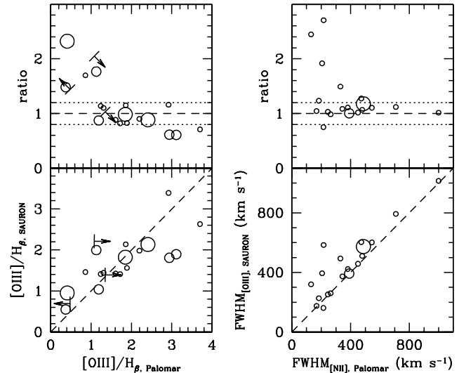
Figure 3. SAURON vs. Palomar. [O III]/ H\beta line ratio (left) and intrinsic width (right) of the [N II] lines from the nuclear spectra of Ho et al. (1997b) compared to [O III]/ H\beta ratio and intrinsic width of the [O III] lines measured with SAURON in the same apertures. The lower panels show the two sets of data directly against each other, while the upper panels show their ratio. Larger symbols correspond to less accurate measurements from Ho et al., while the arrows correspond to upper and lower limits from the same work. The dashed lines show the identity relation, while the dotted lines in the top panels define the region where the SAURON and Palomar measurements agree to within 20%.
