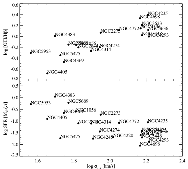
Figure 5. [O\text{ III}]/H\beta ratio and star-formation rate versus H\beta velocity dispersion. Galaxies displaying low velocity dispersions also show the lowest values of [O\text{ III}]/H\beta , suggesting a link between the level of star formation and the dynamical state of the gas. This is confirmed in the bottom panel where the higher star formation rates are found in galaxies with lowest H\beta velocity dispersion.
