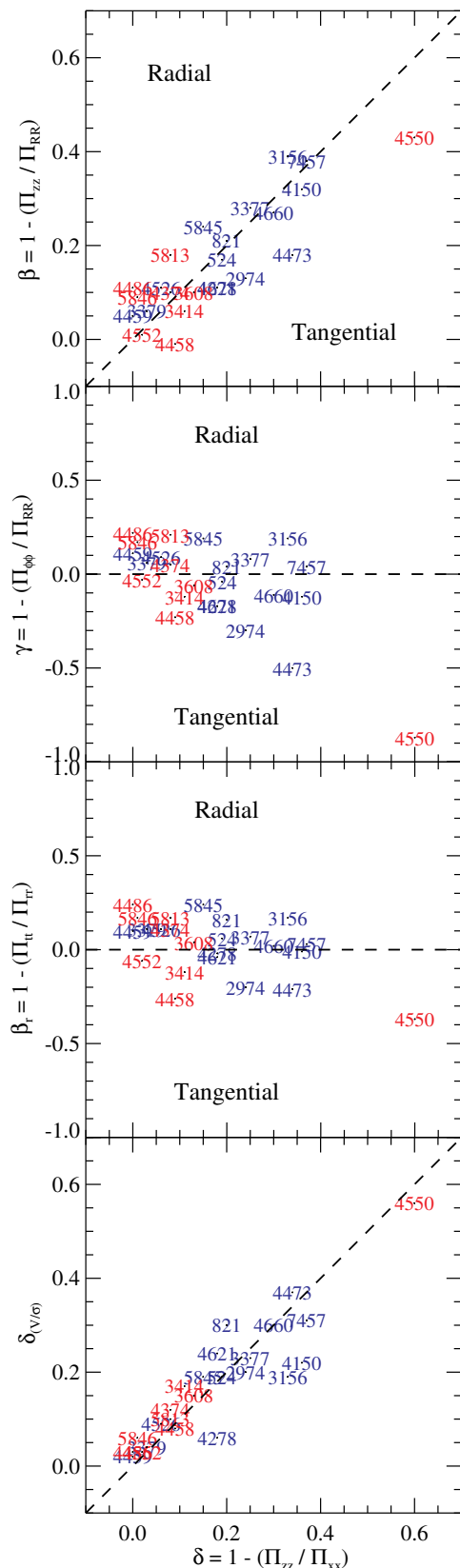
Figure 2. Global anisotropy from the dynamical models. Comparison between the anisotropy \delta determined from the 24 Schwarzschild models of Fig. 1 and the anisotropy parameter \beta (Top Panel), \gamma (Second Panel) and \beta_r (Third Panel). Bottom Panel: Comparison between \delta from the models and \delta_{(V/\sigma)} from the (V/\sigma, \varepsilon) diagram of Fig. 3, after correction for the inclination. The red and blue labels refer to the slow and fast rotators respectively.
