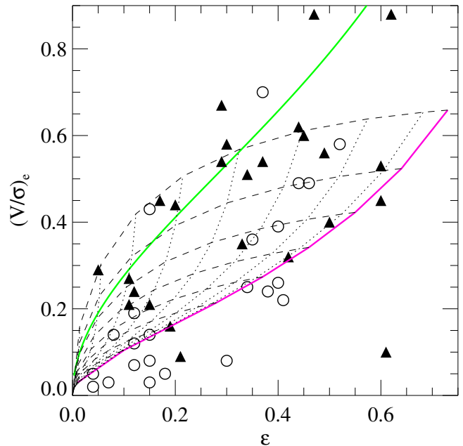
Figure 10. Galaxy morphology on the (V/\sigma, \epsilon) diagram. Same as Fig. 9 but here filled triangles represent S0 galaxies and open circles Es. The envelope of the fast-rotators is populated mainly by S0 in the upper part and by E in the lower part.
