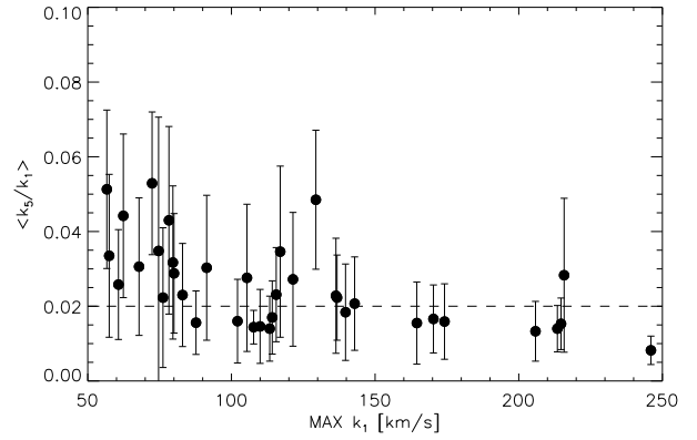
Figure 2. A relation between the maximum amplitude of rotation and luminosity-weighted average of k_5/k_1 ratio, which measures departures from the cosine law for velocity profiles extracted along the best fitting ellipse. All points belong to fast rotators.
