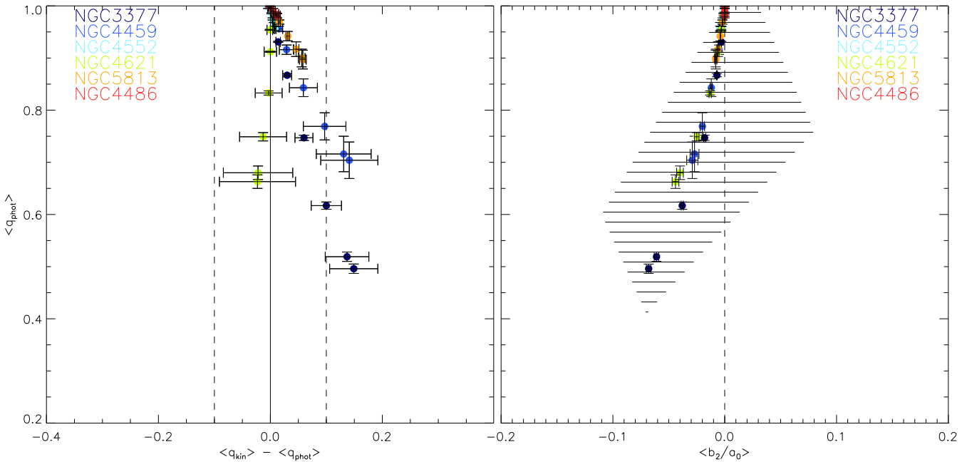
Figure 8. Left: Difference between luminosity weighted kinematic and photometric axial ratio, \langle q_{kin} \rangle and \langle q_{phot} \rangle , for 5 Jeans models at 25^\circ , 35^\circ , 50^\circ , 65^\circ , 80^\circ and 90^\circ inclinations plotted against the luminosity weighted photometric axial ratio. The increase in inclination decreases \langle q_{phot} \rangle and moves points downwards. The vertical dashed lines are guidelines of the variation of q_{kin} profiles from the SAURON data as in Fig. 4. Vertical solid line shows the location of zero difference between \langle q_{phot} \rangle and \langle q_{kin} \rangle . Right: Relation between photometric axial ratio and absolute \langle b_2/a_0 \rangle_\sigma for the same Jeans models as on the left. With increasing inclination the points move towards more negative \langle b_2/a_0 \rangle_\sigma values. The hatched area represents the location of the data from Fig. 5
