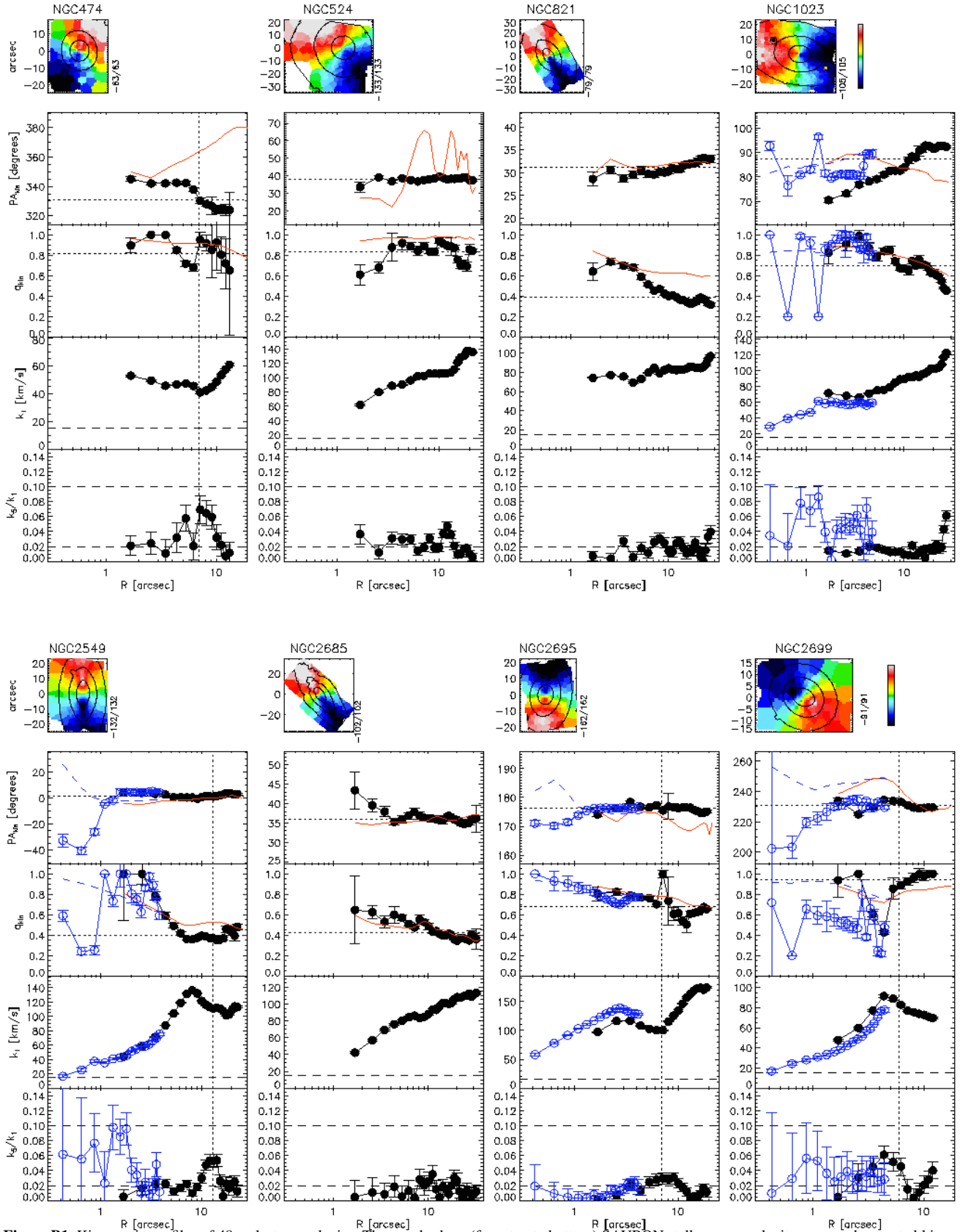
Figure B1. Kinematic profiles of 48 early-type galaxies. The panels show (from top to bottom) SAURON stellar mean velocity map, and extracted kinematic properties: position angle, axial ratio, k_1 and k_5/k_1 coefficients. Solid black symbols are SAURON data, open blue circles are OASIS data. Solid light-blue and green symbols are results of kinemetry on circles for OASIS and SAURON data, respectively. Red line shows photometric PA_{phot} and q_{phot} from the SAURON reconstructed images. Dashed-blue line shows photometric PA_{phot} and 1 - \epsilon from the OASIS reconstructed images. Dashed horizontal lines on k_1 and k_5/k_1 panels show the limiting cases: k_1 = 15 \text{ km s}^{-1} limit of detectable rotation, k_5/k_1 = 0.02 limit of detectable deviation from the assumed cosine function in kinemetry, k_5/k_1 = 0.1 limit for doing kinemetry on circles. These limits are data dependent (for more details see Section 4). Dashed lines \langle q_{kin} \rangle and \langle q_{kin} \rangle show luminosity weighted average values of the radial profiles. In the case of global \langle q_{kin} \rangle innermost 5'' are excluded due to the seeing effects.
