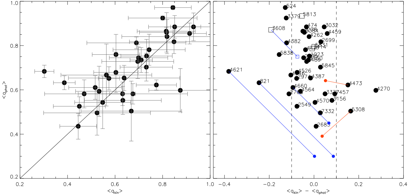
Figure 4. Left: Relation between luminosity-weighted kinematic and photometric axial ratios, \langle q_{kin} \rangle and \langle q_{phot} \rangle , respectively, for fast rotating galaxies in the SAURON survey measured beyond 5'' to avoid seeing effects. The black line is the 1:1 relation. The error bars describe the radial variations of q_{phot} and q_{kin} profiles. Right: Difference between luminosity-weighted kinematic and photometric axial ratios plotted against the photometric axial ratio. Dashed vertical lines represent a typical variation of q_{kin} profiles, which is the dominant uncertainty factor for comparison with q_{phot} . Solid symbols are fast rotating galaxies, while open squares are KDC components of slow rotators. The red lines between symbols link \langle q_{kin} \rangle with \langle q_{phot} \rangle measured on inner (NGC4473) and outer (NGC5308) kinematic components. The blue lines link \langle q_{kin} \rangle and axial ratio of the MGE models.
