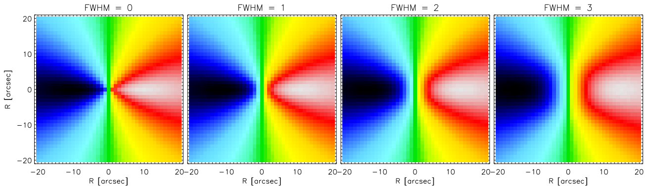
Figure A1. An example of model velocity maps for a given inclination and convolved with different seeing kernels. From left to right: A model velocity map at axial ratio of 0.5 prior to convolution with seeing. Model velocity maps convolved with 1'' , 2'' and 3'' FWHM seeing, respectively. Note the change in the iso-velocity contours in the centre with the increasing seeing.
