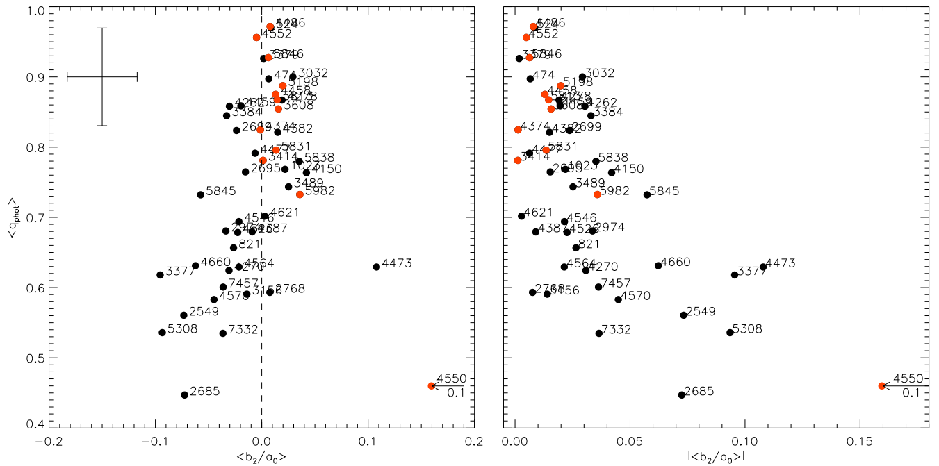
Figure 5. Left: Relation between isophotal axial ratio and the luminosity weighted average normalised second term ( \langle b_2/a_0 \rangle_\sigma ) of the Fourier decomposition of the velocity dispersion profiles extracted along the isophotes. Red symbols are slow rotators. An average uncertainty, describing the radial variation of b_2/a_0 profiles, is shown in the upper left corner. Large negative \langle b_2/a_0 \rangle_\sigma values are typical for iso- \sigma contours that are rounder than the isophotes, while large positive \langle b_2/a_0 \rangle_\sigma values are typical for flatter iso- \sigma contours than the isophotes. Right: same as left, but now absolute values of \langle b_2/a_0 \rangle_\sigma are plotted. In both images, NGC4550 was shifted to the left for 0.1 for presentation purposes, as shown by the arrows.
