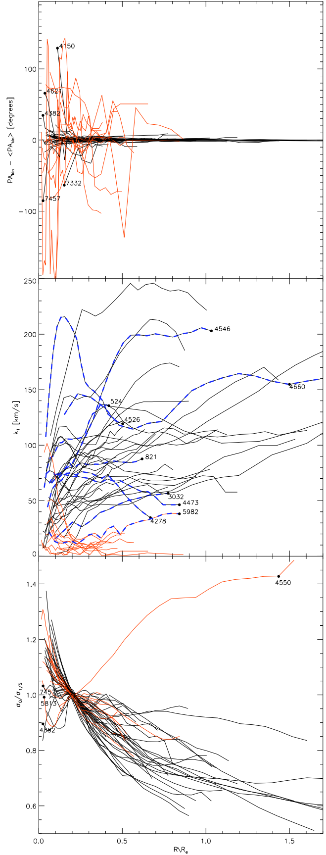
Figure 3. Radial profiles of (from top to bottom) \text{PA}_{kin} - \langle \text{PA}_{kin} \rangle , k_1 and \sigma_0 from the SAURON data. \langle \text{PA}_{kin} \rangle are luminosity weighted averages of \text{PA}_{kin} profiles. \sigma_0 profiles are normalised at R_e/5 . The profiles of slow and fast rotators are coloured in red and black, respectively. In the middle panel dashed blue lines are over-plotted to guide the eye for the cases with specific profiles as mentioned in text.
