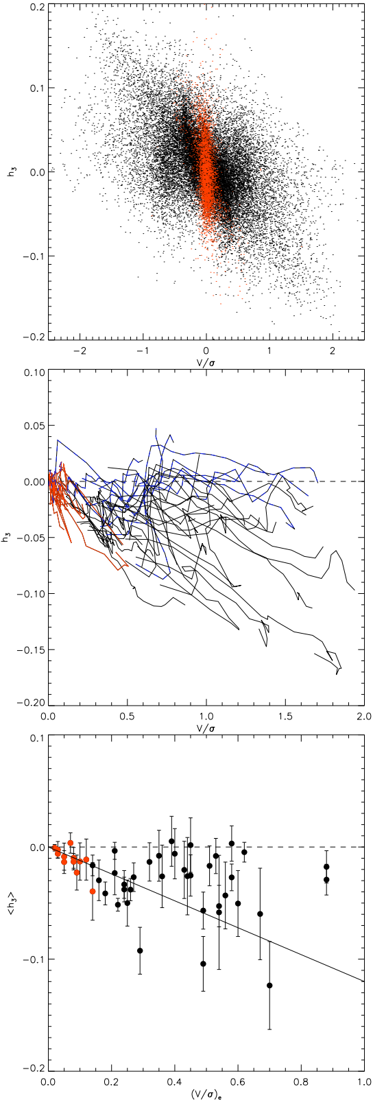
Figure 6. Top: Local h_3 - V/\sigma relation for all data points of the 48 SAURON galaxies with h_3 error less than 0.2. Middle: Profiles of h_3 - V/\sigma relation averaged on ellipses. On all maps ( V , \sigma and h_3 ) profiles were extracted along the best fitting ellipses to the velocity maps. Typical error bars are of the order of 0.01 or smaller, due to averaging along the best fitting ellipse. Bottom: Relation between the luminosity averaged h_3 and (V/\sigma)_e ( V/\sigma within 1 R_e from Paper X). The error bars describe the radial variation of h_3 profiles. The solid line is the relation from Bender et al. (1994). On all panels, slow rotators are shown in red. © 2007 RAS, MNRAS 000, 1–20
