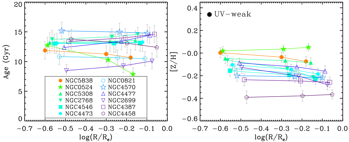
Figure 14. Same as Figure 13 but for UV-weak galaxies.
