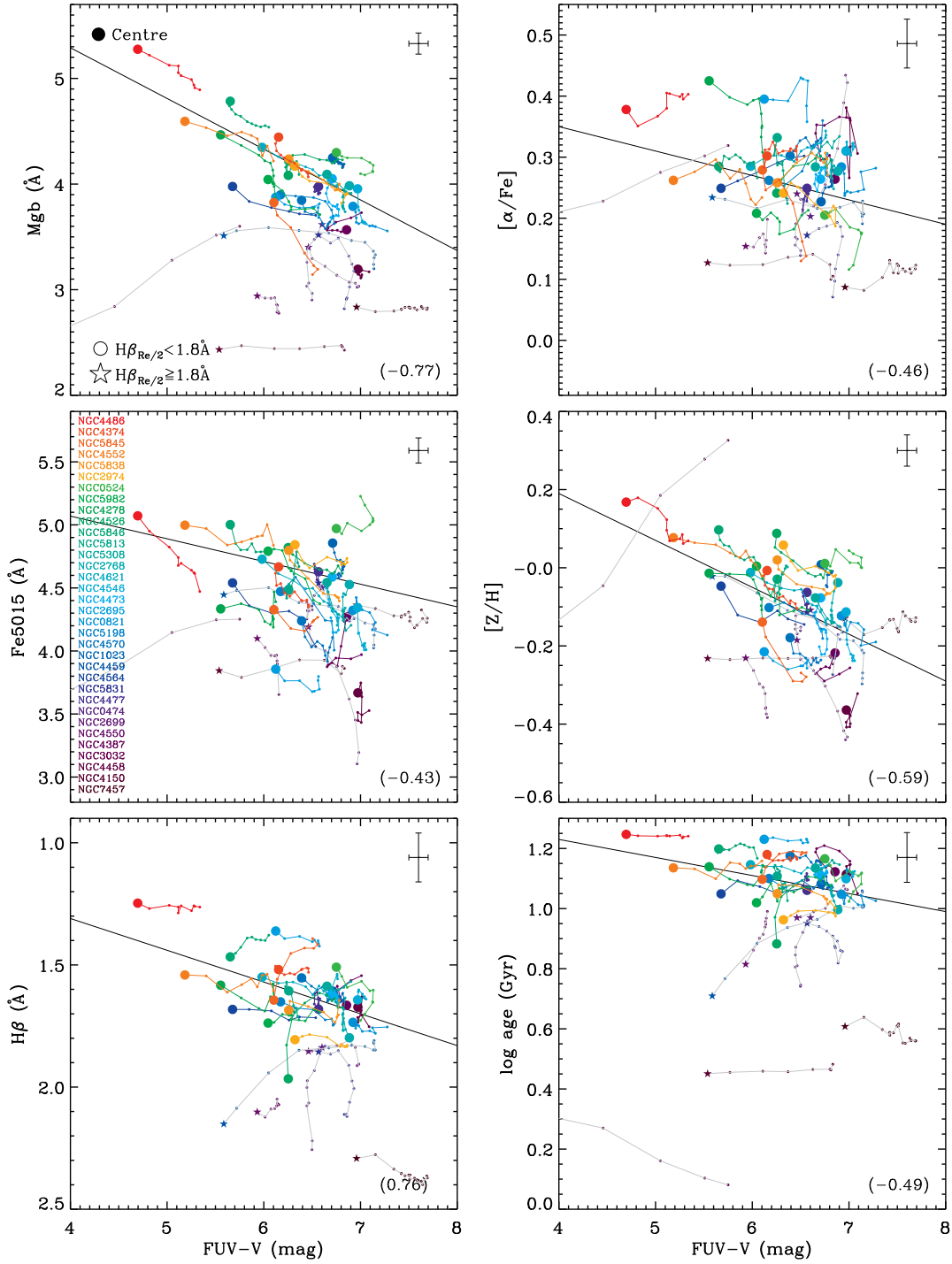
Figure 1. UV upturn dependence on measured line strengths and derived stellar population properties. The Mgb ( top-left ), Fe5015 ( middle-left ), H\beta ( bottom-left ), [\alpha/\text{Fe}] ( top-right ), [Z/H] ( middle-right ) and age ( bottom-right ) parameters are shown as a function of the FUV-V colour. We note that all line strengths and derived stellar population properties are based on the SAURON data published in Paper VI and Paper XVII, respectively. The sample is divided into quiescent early-type galaxies (circles, H\beta_{Re/2} \leq 1.8 \text{ \AA} ) and galaxies with recent star formation (stars, H\beta_{Re/2} > 1.8 \text{ \AA} ). The solid line in each panel is a linear fit to all of the quiescent galaxy profiles, weighting each radius by its V-band luminosity, and the correlation coefficient is reported in the bottom-right corner. The symbols are colour-coded according to the integrated stellar velocity dispersion within one effective radius ( \sigma_e ). All the points for an individual galaxy are represented by a single colour, and the symbol for the central point is larger.
