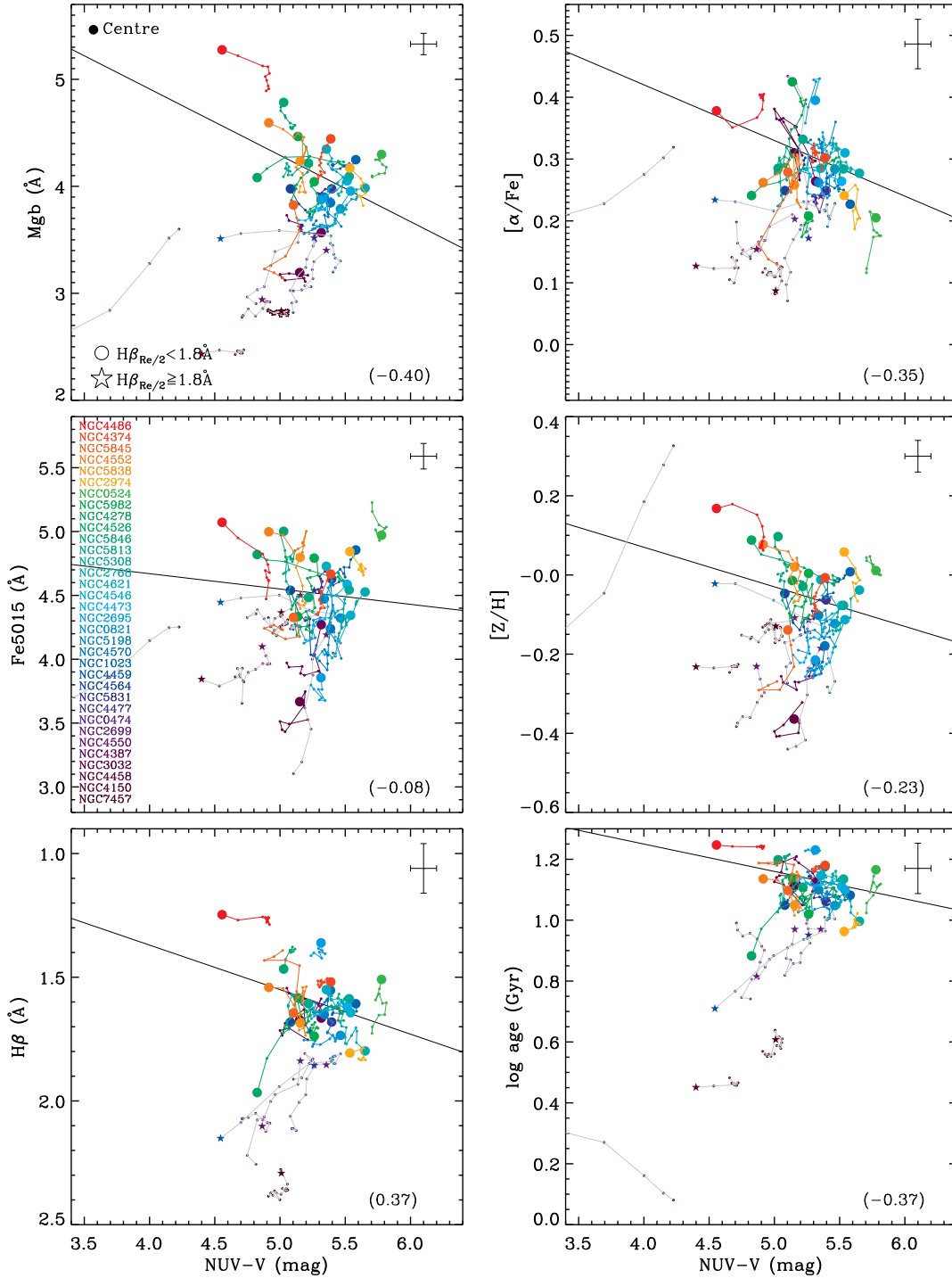
Figure 2. Same as Figure 1 but for the NUV-V colour.
