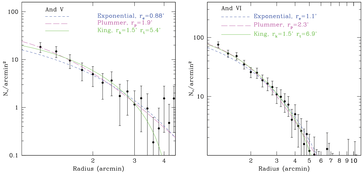
Figure 2. Radial profile for And V (left) and And VI (right) constructed from aperture star counts in the region of both dSph. In each case, an average background number density was estimated from an annulus located between 8 and 12 arcmin from the centre of each object, and the results were subtracted from our star counts. We overlay the best-fitting Exponential (blue short dashed line), Plummer (magenta long-dash line) and King (green solid line) profiles in each case also.
