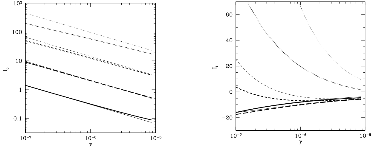
Figure 7. As Fig. 6, but for injection at line centre. Here the approximate versions include terms up to order \beta .
