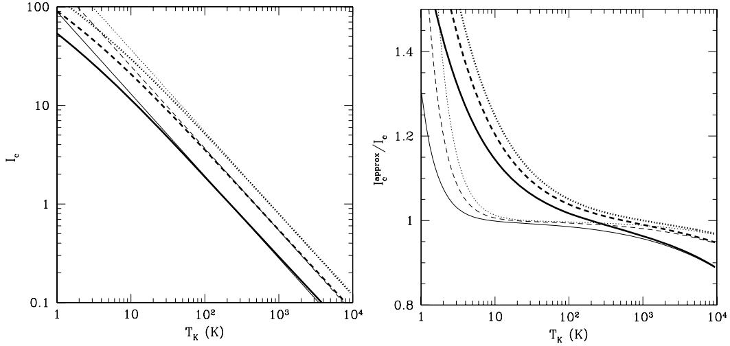
Figure 5. Heating integral for continuous injection. Left-hand panel: the thick solid, dashed and dotted curves show I_c for a Voigt profile at z = 10, 20 and 30 . The thin curves show the corresponding quantities using only the first-order term in equation (31). Right-hand panel: ratio of the power series approximation to I_c (using the wing approximation) to the exact value. The thick and thin curves retain terms to order \beta and \beta^3 , respectively.
