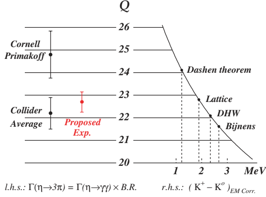
Figure 24: Quark-mass ratio \mathcal{Q} as determined from \eta decay and from K^+ - K^0 mass difference. Indicated in red is the projected uncertainty from the proposed measurement of \Gamma_{\eta \rightarrow \gamma\gamma} . Figure adapted from H. Leutwyler [Le96].
