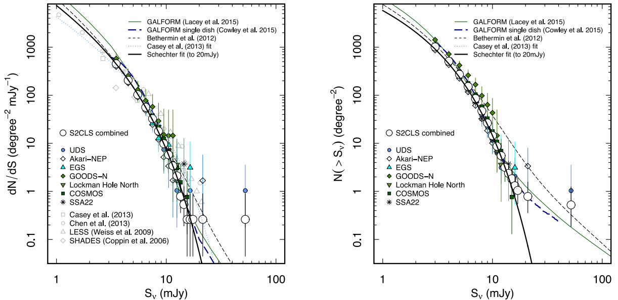
Figure 15. Number counts of 850 \mu m sources. The left-hand panel shows the differential number counts for individual fields and the combined survey, along with a selection of data from the literature. Two model curves show the parametric evolving luminosity function model of Béthermin et al. (2012) and the semi-analytic (GALFORM) model of Lacey et al. (2016). The Cowley et al. (2015) line shows the same GALFORM model but taking into account source blending due to the 15 arcsec JCMT beam. The presence of foreground sources and the effect of gravitational lensing causes an upturn in the counts at bright flux densities at a level in reasonable agreement with the models (note that the GALFORM model does not include lensing) given the low number statistics at these bright flux densities. For clarity, we only show error bars for the S2CLS data, which are evaluated from Poisson statistics (Gehrels 1986). The right-hand panel shows the cumulative counts where, for clarity, we only plot the S2CLS data, fit, and models.
