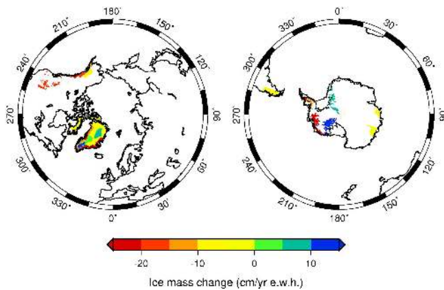
Fig. 1. Spatial distribution of ice mass trends for the regions listed in Table 1 for the period 2000–2008.
