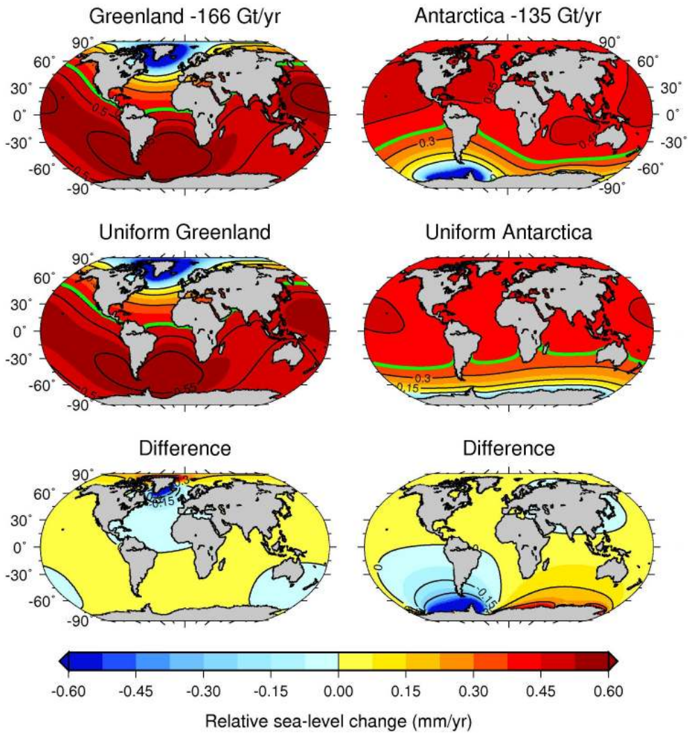
Fig. 3. Impact on relative sea level assuming uniform mass loss over Greenland, and the whole of Antarctica compared with the distribution shown in Fig. 1. The top panel is the same as Fig. 2a and b; the middle panel is for mass loss uniformly distributed across the ice mass and the bottom panel the difference between the two (observed-uniform).
