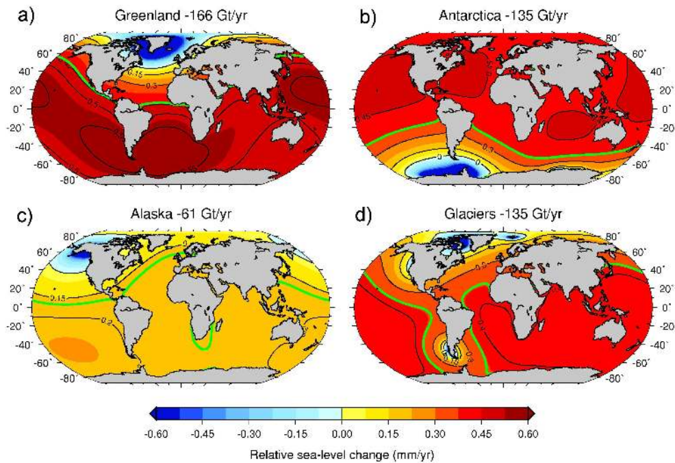
Fig. 2. Relative sea level variations due the gravitational and Earth rotational effects of ice mass losses from different sources for the period 2000–2008 inclusive; (a) Greenland, (b) Antarctica, (c) Alaska, (d) mountain glaciers and ice caps in the Arctic, Patagonia and Rockies. The thick green contour indicates the global average eustatic RSL for each source.
