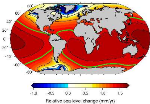
Fig. 4. The combined relative sea level variations for all ice masses. The thick green contour indicates the global average eustatic RSL (1.4 mm yr -1 ).
