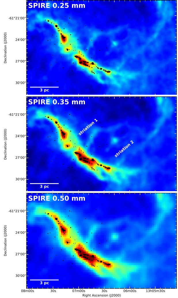
Fig. 2. Herschel /SPIRE images of G304.74 and its surroundings. The images are displayed in logarithmic colour-scale to improve the appearance of the low surface brightness features. The overlaid black contours show the SABOCA 350 \mu\text{m} dust continuum emission as in Fig. 1. A scale bar of 3 pc projected length is shown in the bottom left corner of each panel . The two obvious striations are labelled in the middle panel (striation 1 and striation 2).
