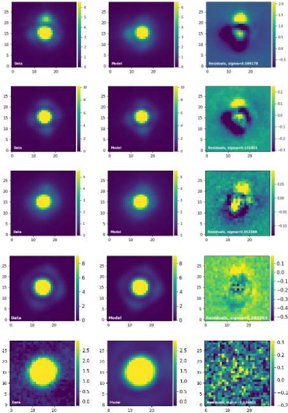
Fig. 7. From the top: epoch 1 (2015-10-26), epoch 2 (2015-12-19), epoch 3 (2018-12-16) in H2 -band, and epoch 4 (2020-01-05) in K1 -band for DH Tau B as observed with SPHERE/VLT, and the observation (2019-09-19) in the L' -band obtained with LMIRCam/LBTI. The candidate companion is visible in the right panels of the SPHERE observations. There is no detection for the LBT data.
