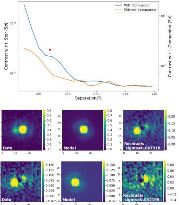
Fig. B.6. Contrast curve ( upper figure ) with and without the P2 point source (S2 was removed before calculating the contrasts and is represented by the red dot) and images of the object P2 ( lower figures ) around HIP 87836, model and residuals of, from the top , the primary P2, and the secondary S2.
