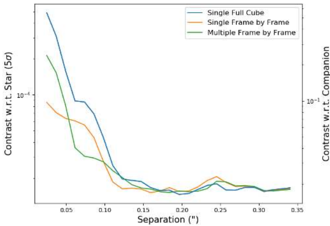
Fig. 4. Contrast curve around HD 1160 B using one single model PSF with the single_fullcube (blue curve) and single_framebyframe (orange curve) routines, and multiple model PSFs using HD1160 C in place of the star for the multiple_framebyframe routine (green curve). Contrasts are calculated with respect to the central star on the left y -axis and with respect to HD 1160 B on the right one.
