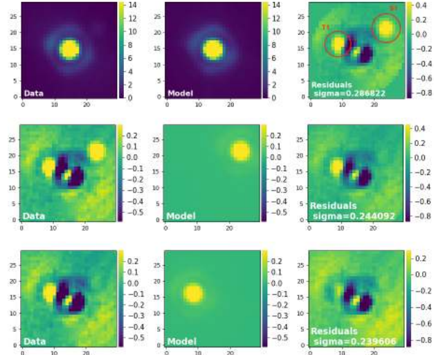
Fig. B.5. Images of the object P1 around HIP 87836, model and residuals of, from the top , the primary P1, the secondary S1, and the tertiary T1.
