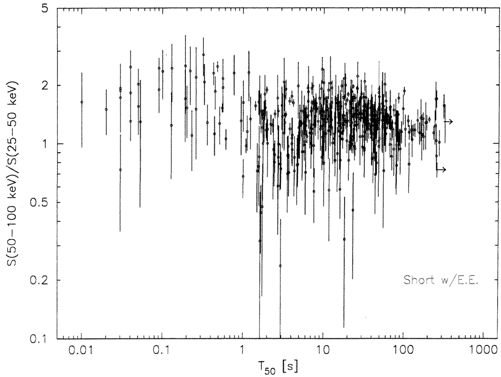
Fig. 8.— The fluence ratio between the 50-100 keV and the 25-50 keV bands and T_{90}(top) and T_{50}(bottom) . Short GRBs with an E.E. are shown in red.
