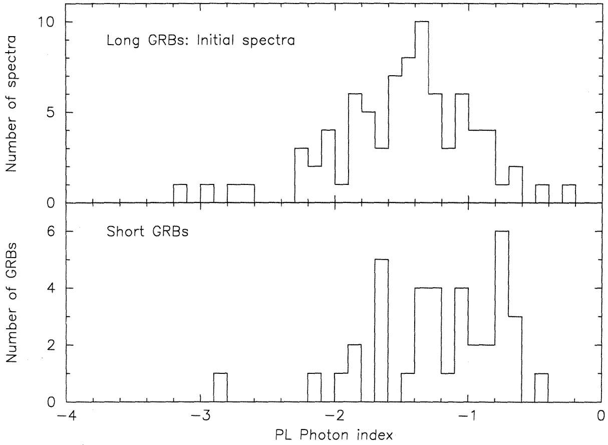
Fig. 18.— Histograms of the BAT photon index in a PL fit for initial spectra of long GRBs (top) and for short GRBs (bottom).
