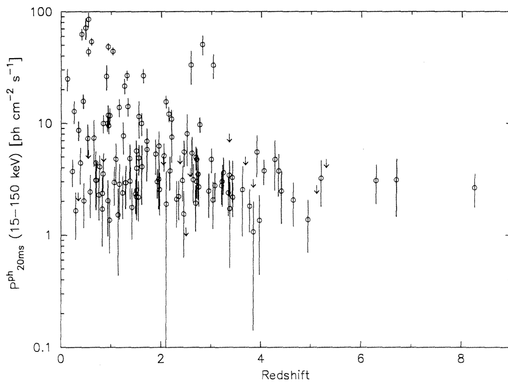
Fig. 29.— Distribution of 1 s (top) and 20 ms (bottom) observed peak photon flux in the 15-150 keV band vs. redshift.
