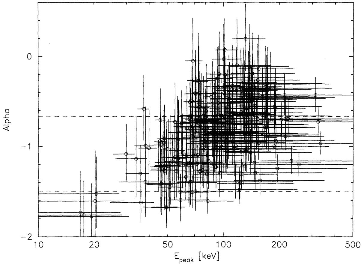
Fig. 20.— Distribution of the BAT photon index \alpha and E_{\text{peak}} in a CPL fit. The red dashed lines show the photon index region from -3/2 to -2/3 . The total number of time-resolved spectra is 234.
