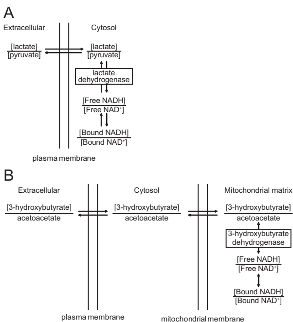
FIG. 4. Metabolite indicators for NAD^+/NADH . A, Lactate dehydrogenase as specific metabolite indicator reaction for cytosolic NAD^+/NADH . B, Mitochondrial 3-hydroxybutyrate dehydrogenase as a specific metabolite indicator reaction for mitochondrial NAD^+/NADH .
