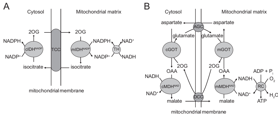
FIG. 6. Redox shuttles. A, Schematic description of the NADP(H) redox shuttle: the NADPH as produced in the transhydrogenase (TH) reaction is transduced to the cytosol via the 2-oxoglutarate (2OG)–isocitrate redox shuttle in which mitochondrial NADPH first reacts with 2-oxoglutarate and bicarbonate as catalyzed by the mitochondrial NADP-linked isocitrate dehydrogenase (mIDH NADP ) to produce isocitrate and NADP + , followed by the export of isocitrate to the cytosolic in exchange for 2-oxoglutarate. The isocitrate now present in the cytosol space is then converted back into 2-oxoglutarate and bicarbonate via the cytosolic NADPH-linked isocitrate dehydrogenase (cIDH NADP ), followed by the uptake of 2-oxoglutarate into the mitochondrial space in exchange for isocitrate. TCC, Tricarboxylate. B, Schematic description of the malate/aspartate NAD(H)-redox shuttle. The NADH that is produced in the cytosol, for instance during glycolysis, is first converted into malate via cytosolic NAD + -linked malate dehydrogenase (mMDH NAD ), after which the malate is transported into the mitochondria in exchange for 2-oxoglutarate (2OG). Intramitochondrial malate is then converted into oxaloacetate (OAA), during which NADH is generated, which can now be used in the respiratory chain (RC) with formation of ATP. The oxaloacetate is not very permeable to mitochondrial membranes and is therefore first converted into aspartate via the glutamate oxaloacetate transaminase (GOT; cGOT, cytosolic GOT; mGOT, mitochondrial GOT), followed by the export of aspartate in exchange for glutamate. Cytosolic aspartate is subsequently converted back into cytosolic oxaloacetate, thus completing the cycle. Note that cytosolic NADH can also be reoxidized via other redox shuttles including the \alpha -glycerol-3-phosphate shuttle in which the NADH first reacts with dihydroxyacetonephosphate to generate glycerol-3-phosphate plus NAD + , after which glycerol-3-phosphate directly transfers its electrons to the respiratory chain at the level of ubiquinone via the membrane-bound enzyme \alpha -glycerol-3-phosphate dehydrogenase, thus completing the cycle. DCC, Dicarboxylate carrier; AGC, aspartate-glutamate carrier.
