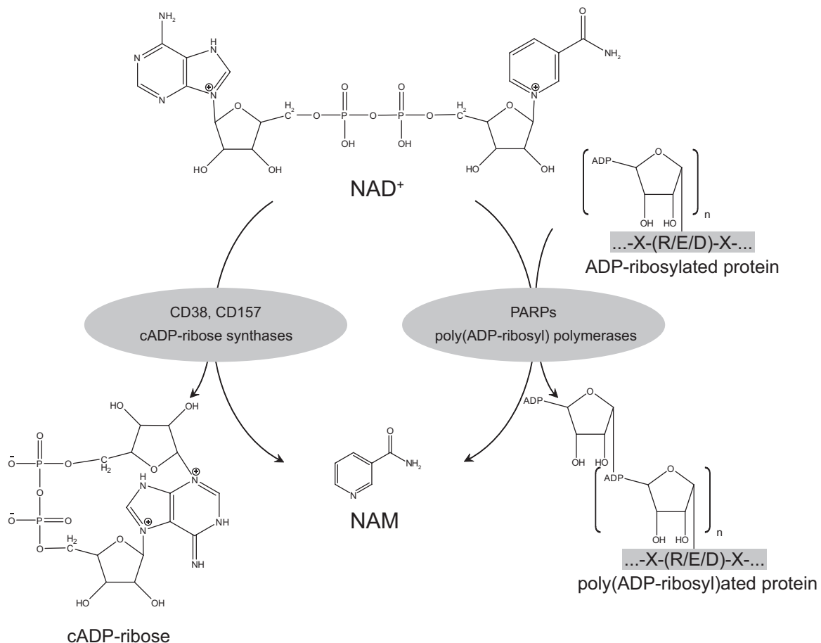
FIG. 9. PARPs and cADP-ribose synthases as NAD + -consuming enzymes. Intracellular NAD + content largely depends on the activities of two different families of enzymes: PARPs and cADP-ribose synthases (CD38 and CD157), both of which render NAM as an end-product. PARPs catalyze a reaction in which the ADP-ribose moiety is transferred to a substrate protein. PARPs can transfer multiple ADP-ribosyl groups and form long chains and branches of ADP-ribosyl polymers. cADP-ribose synthases use NAD + to generate cADP-ribose, which acts as an intracellular secondary messenger.
