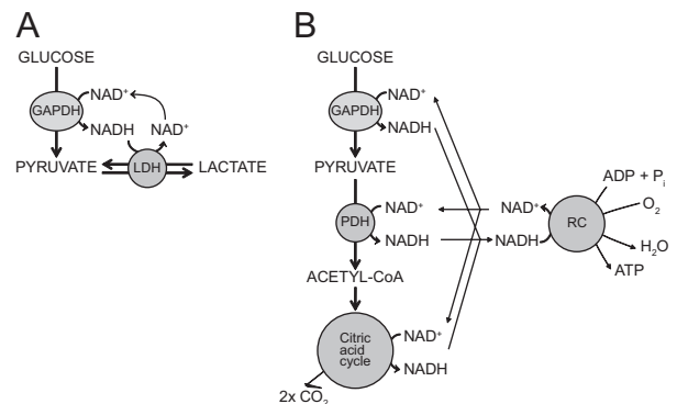
FIG. 7. Regulation of mitochondrial and cytosolic redox state. A, Anaerobic metabolism of glucose into lactate with NADH produced in the glyceraldehyde-3-phosphate dehydrogenase (GAPDH) reaction and with lactate dehydrogenase (LDH) reconverts NADH back into NAD + . B, Schematic representation of the aerobic oxidation of glucose with particular attention for the sites at which NADH is formed including: 1) the GAPDH reaction during glycolysis; 2) the pyruvate dehydrogenase (PDH) complex; and 3) the citric acid cycle, followed by the reoxidation of NADH back to NAD + by the respiratory chain (RC) with the concomitant formation of ATP from ADP + phosphate.
