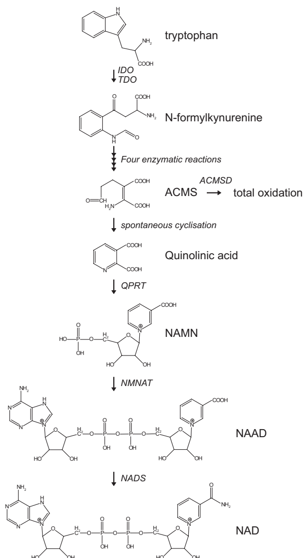
FIG. 1. De novo \text{NAD}^+ biosynthesis from tryptophan. The de novo biosynthesis of \text{NAD}^+ starts with the conversion of tryptophan to N-formylkynurenine catalyzed by either IDO or TDO. N-Formylkynurenine is subsequently converted in four individual steps to the unstable ACMS, which can undergo either enzymatic conversion directed to total oxidation or nonenzymatic cyclization to quinolinic acid. The final step of the dedicated de novo biosynthesis of \text{NAD}^+ is comprised of the QPRT-catalyzed formation of NAMN. NAMN is subsequently converted to NAAD by one of the NMNAT enzymes. The final step in the biosynthesis of \text{NAD}^+ is the amidation of NAAD by the NAD synthase enzyme.
