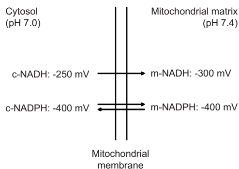
FIG. 3. Redox potentials of the mitochondrial and cytosolic NAD(H) and NADP(H) systems in the liver. c, Cytosolic; m, mitochondrial.
