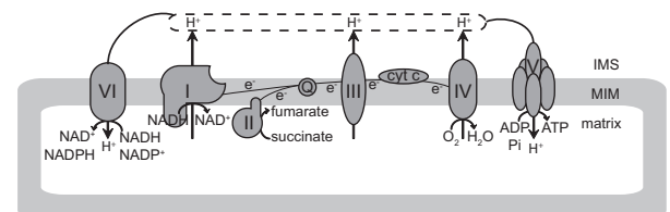
FIG. 5. The role of the energy-linked transhydrogenase for the redox state. Schematic representation of the mitochondrial respiratory chain system, including complex VI, which is the energy-linked transhydrogenase catalyzing the reaction: NADH + NADP^+ \leftrightarrow NAD^+ + NADPH . The fact that complex VI is driven by the proton gradient across the mitochondrial membrane (just like the F_1F_0 -ATP-ase) drives the transhydrogenase reaction far to the site of NADP reduction so that the transhydrogenase reaction is virtually unidirectional ( NADH + NADP^+ \rightarrow NAD^+ + NADPH ). MIM, Mitochondrial inner membrane; cytc, cytochrome c; IMS, intermembrane space.
