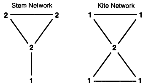
Figure 2. Initial GPI Values for Stem and Kite Networks
