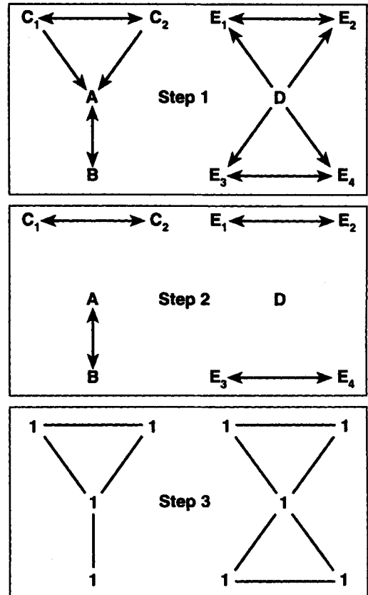
Figure 3. Iterative Analysis for Computation of GPI_2 for Stem and Kite Networks
