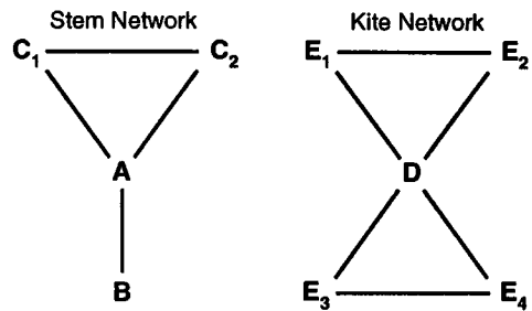
Figure 1. The Stem and Kite Networks
