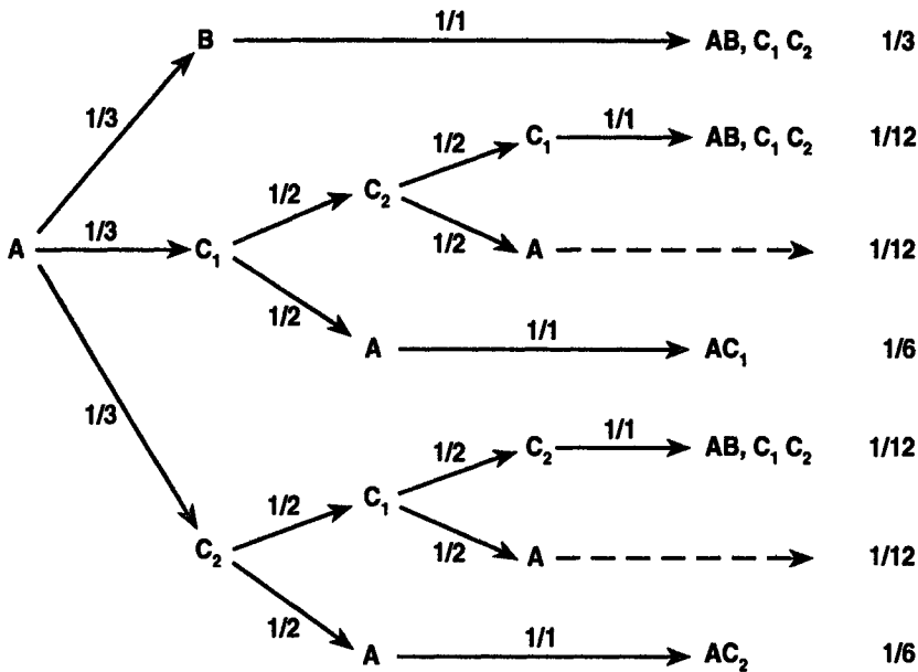
Figure 4. Tree Diagram for Computing GPI_3 for the Stem Network
