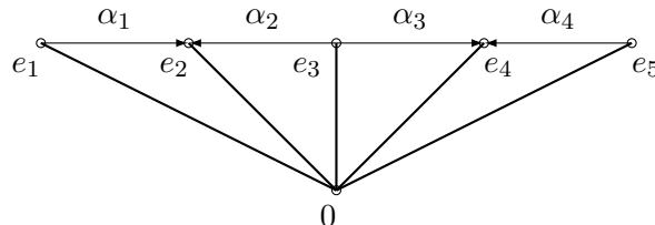
Figure 4: \Delta_4 as a semigroup of mappings.
