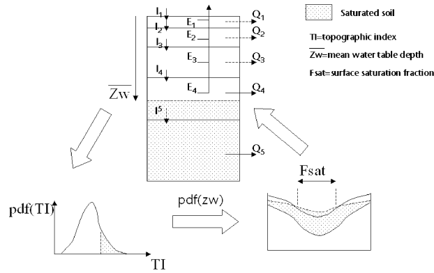
FIG. 1. Schematic diagram of the combined MOSES-TOPMODEL approach.
