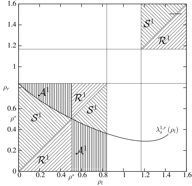
FIGURE 6. Classical 1-waves: density components of states (\rho_l, v_l) and (\rho_r, v_r) within one phase can be connected by a classical 1-wave. \mathcal{S}^1 corresponds to an 1-shock wave (cf. Lem. 2.6), \mathcal{R}^1 to a 1-rarefaction wave (cf. Lem. 2.9) and \mathcal{A}^1 to an attached 1-wave (cf. Lem. 2.10).
