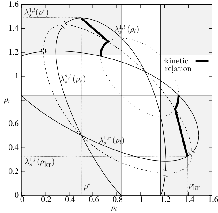
FIGURE 8. The graph of the kinetic relation (bold solid line) is displayed as given in Definition 2.12 is displayed. Furthermore the entropy dissipation curve \Gamma_\Delta (dashed line), and the characteristic curves (solid lines) are shown which impose some restrictions on the choice of the kinetic relation as discussed in Remark 2.13.
