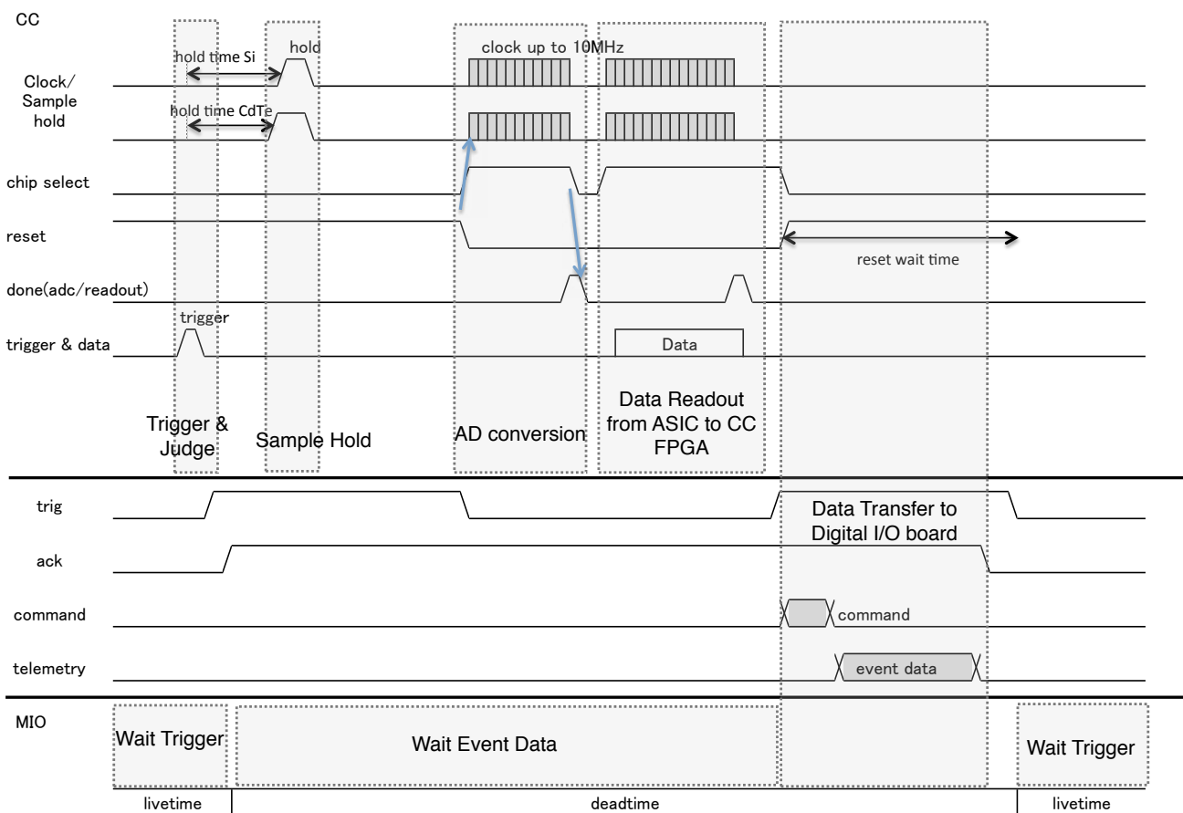
Figure 10: Timing chart representing the readout sequence of the SGD Compton camera.
