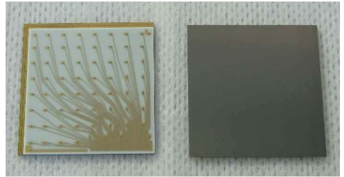
Figure 6: The CdTe pixel sensor devices bonded with the ceramic fanout board. The left half shows the front with the ceramic fanout board for the pixels and the right half shows the common anode electrode utilizing Indium.
