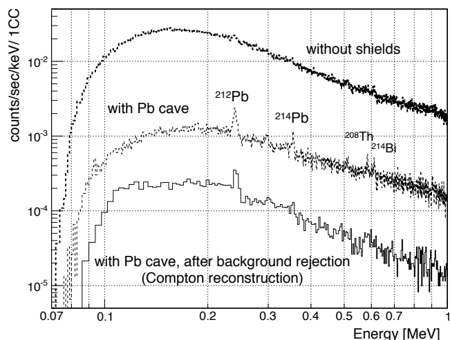
Figure 14: Background spectra obtained with the prototype SGD Compton camera. The room background spectrum obtained without any shields, the spectrum with the Pb cave, and the spectrum after the Compton reconstruction are plotted.
