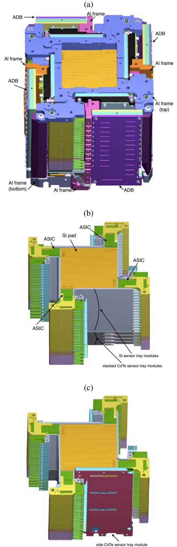
Figure 2: (a) 3D model of Compton camera structure. (b) Si and CdTe stack only. (c) One side CdTe tray module is installed in the stack.
