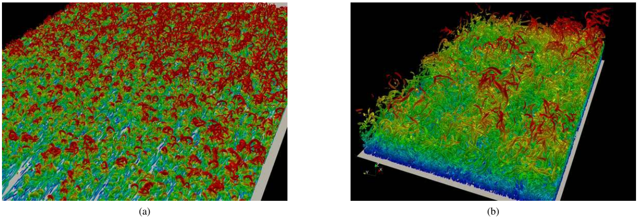
Figure 1. Three-dimensional visualization of vortical structures in a DNS of a turbulent boundary layer at (a) Re_\theta \approx 600 and (b) Re_\theta \approx 4300 [8]. The transitional region is characterized by individual hairpin vortices while no such regularity is evident at higher Re .
