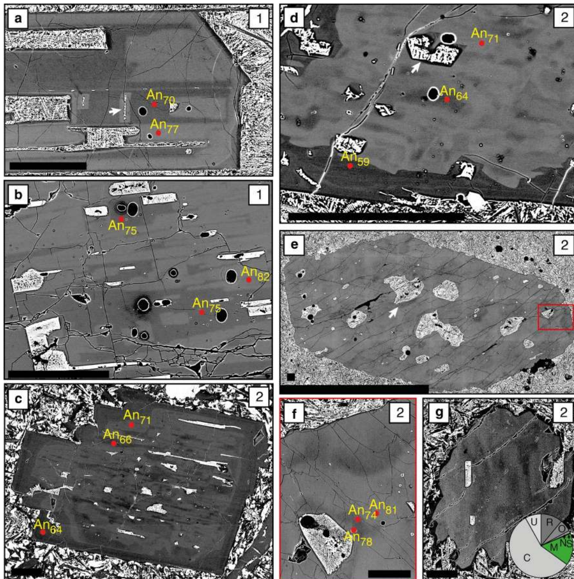
Fig. 8 Type 1 (a, b) and Type 2 (c–g) patchy zoning in plagioclase; the zoning type is indicated in the top right of each panel. a Geometric Type 1 zoning with a skeletal geometric low anorthite core containing patches of higher anorthite similar in composition to the surrounding mantle. b The low anorthite skeletal core contains patches of higher anorthite, and higher anorthite regions also contain low anorthite patches similar in composition to the skeletal core. c Plagioclase exhibiting Type 2 patchy zoning characterised by low anorthite amoeboid patches that show a degree of crystallographic alignment along cleavage planes. These patches have similar anorthite
