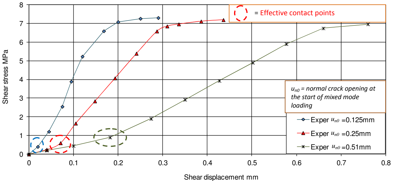
Figure 4. Shear contact transition zones from Paulay and Loeber's tests [6]
