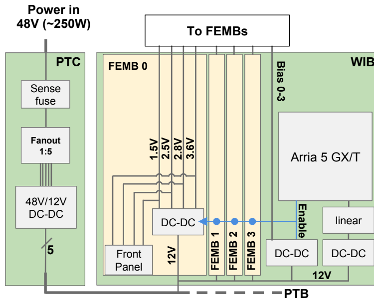
Figure 2.47: LV power distribution to the WIB and FEMBs. 250W is for a fully-loaded crate with the majority of the power dissipated by the 20 cold FEMBs in the LAr.
