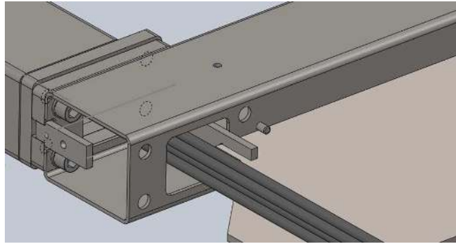
Figure 2.55: Diagram showing the routing of the PDS cables through the APA frame.
