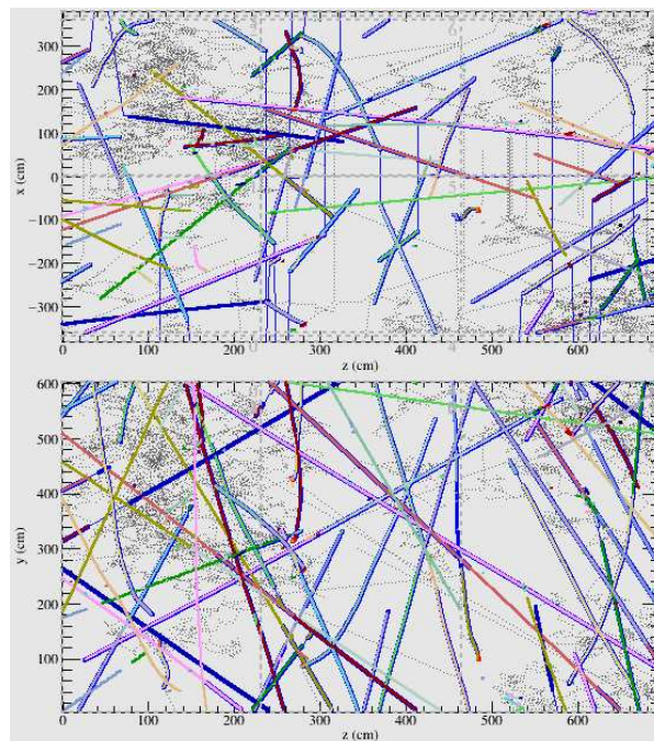
Figure 5.9: Example of reconstructed cosmic muons using gaushit, Line Cluster and PMA.
