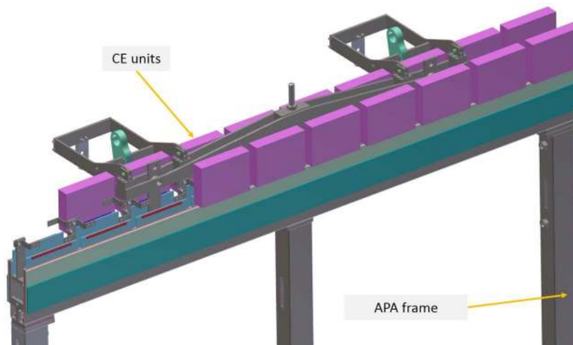
Figure 4.4: CE installation
