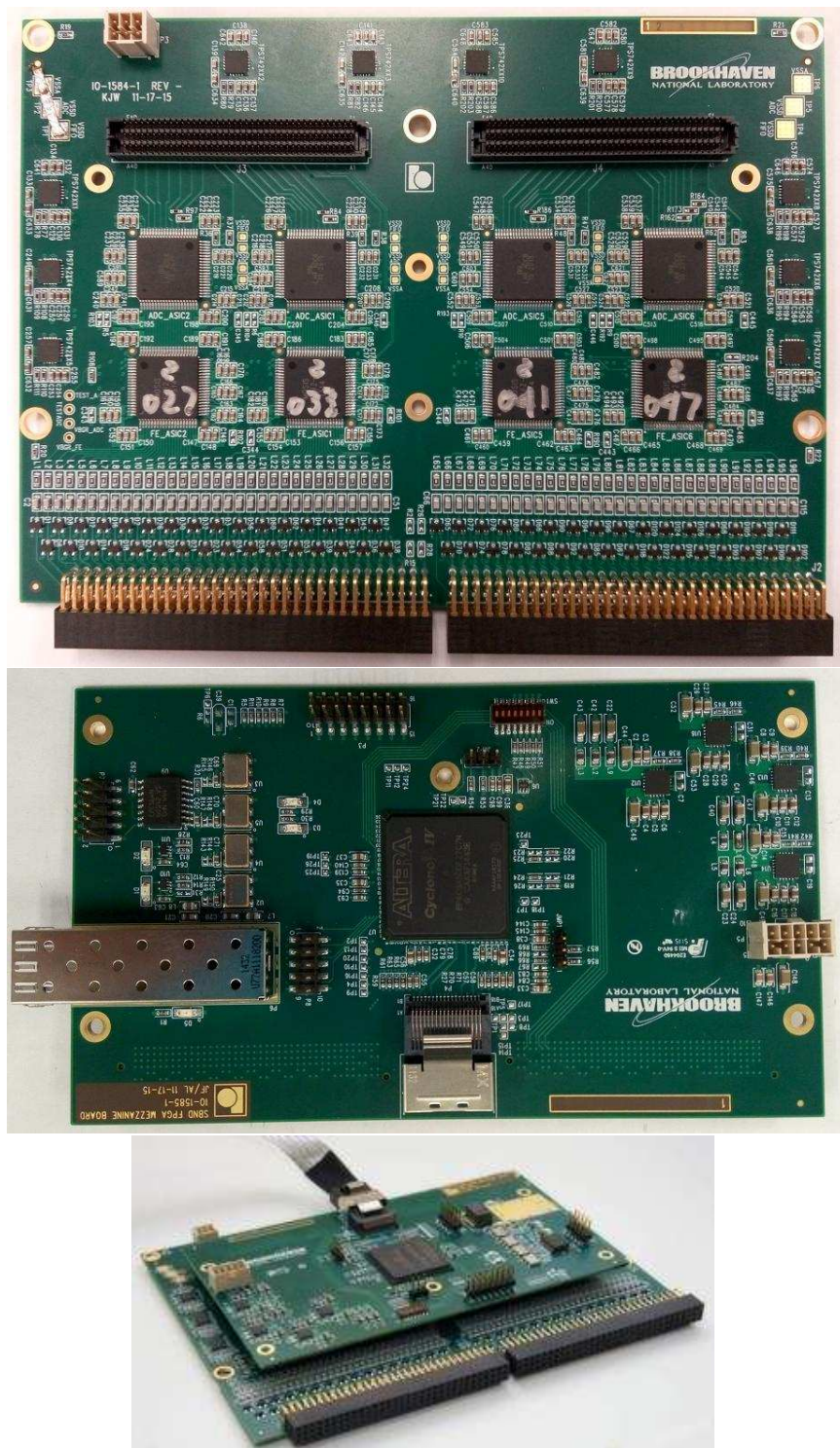
Figure 2.35: The Front End Mother Board (FEMB), as used in the early set of tests. Top: The analog mother board, showing four ADC ASICs and four FE ASICs surface mounted. The other side of the board has another four ADC and FE ASICs. Except for anticipated small modifications, this board is essentially the final version. Middle: The FPGA mezzanine, used in place of the digital ASIC mezzanine for the early set of tests. Bottom: The complete FEMB assembly as used in the early set of tests. The cable shown in the high-speed data, clock, and control cable. The middle and bottom photos are from an SBND version, which uses a different output data connector and a different input connection orientation.
