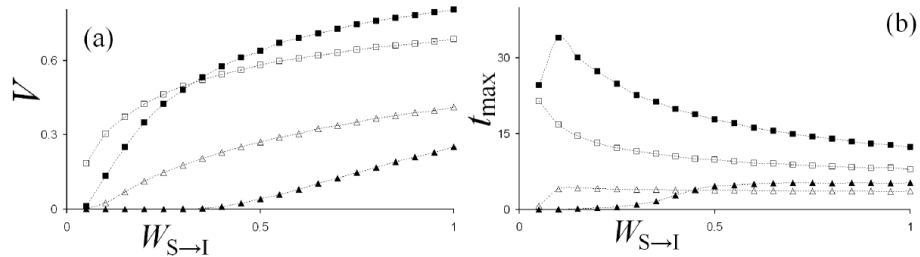
Fig. 1. The influence of the parameter W_{S \to I} on the magnitude of epidemic V (a) and time t_{\max} (b) for different values of W_{I \to R} (0.1 — boxes and 0.9 — triangles). Black and white marks correspond to uniform and real distribution of activity, respectively. Results were averaged over 10^4 independent simulations. The values of the other parameters are: W_{R \to S} = 0 .
