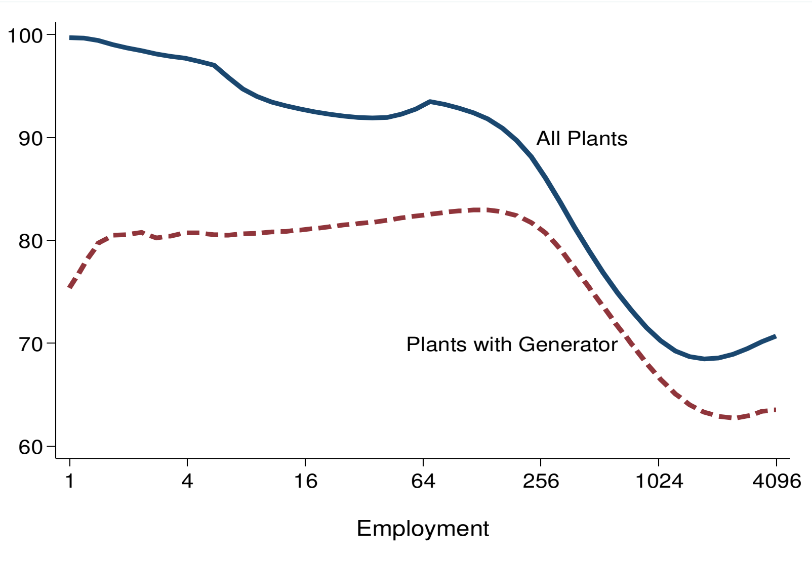
Figure 11: % Electricity Purchased from Grid in India
