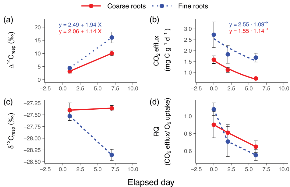
FIGURE 7 Results (mean \pm SE) for coarse roots (> 2 mm) and fine roots ( \leq 2 mm) from repeated respiration incubations during 7 days. (a) the \Delta^{14}\text{C} signature of the respired \text{CO}_2 ( \Delta^{14}\text{C}_{\text{resp}} ). Presented are equations of linear regression models; (b) \text{CO}_2 efflux rates. Presented are equations that best fitted the results to the equation y = a \times b^{-x} ; (c) the \delta^{13}\text{C} signature of respired \text{CO}_2 ( \delta^{13}\text{C}_{\text{resp}} ); (d) RQ (ratio \text{CO}_2 efflux/ \text{O}_2 uptake). Results in panels (a) and (c) were measured in two-day flask incubations ( n = 4, 3 for coarse and fine roots, respectively), results in panels (b) and (d) were measured in short-term incubations ( \sim 20 min, according to the consecutive incubations order, n = 3, 4, 3 for coarse roots, and n = 3, 4, 4 for fine roots) [Colour figure can be viewed at wileyonlinelibrary.com ]
