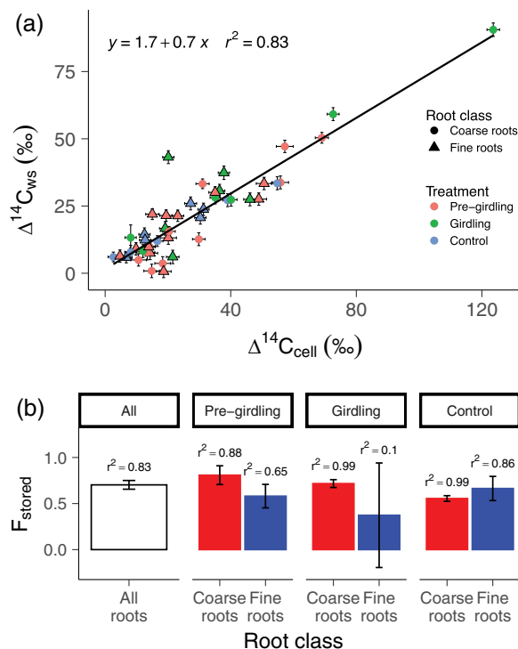
FIGURE 6 (a) A scatter plot of the \Delta^{14}\text{C} signatures of the water-soluble C ( \Delta^{14}\text{C}_{\text{ws}} ) and \alpha -cellulose C ( \Delta^{14}\text{C}_{\text{cell}} ) extracted from roots, with the equation of the linear model for all results pooled together. The shapes indicate the root class (coarse roots, > 2 mm, fine roots, \leq 2 mm), and colours indicate the treatment: before girdling (Pre-girdling), ~3 months after girdling (Girdling) and ~3 months after girdling in un-girdled trees (Control). Error bars are the analytical uncertainty; (b) the stored fraction ( F_{\text{stored}} ) from the total water-soluble C as estimated from the slope when the linear model is applied to the different subgroups ( n = 46, 11, 12, 6, 6, 5, 6 , respectively). For example, the slope in the equation in panel (a) is 0.7 therefore F_{\text{stored}} for the subgroup "All" is 0.7. Labels within the bars are the r^2 of the linear regression. Error bars are the standard error of the slope estimate [Colour figure can be viewed at wileyonlinelibrary.com ]
