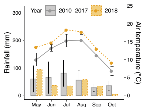
FIGURE 1 Mean monthly rainfall (mm, bars) and air temperature (°C, circles) during 2018 growing season, and in the previous 8 years (2010–2017) in the study site (Großer Hermannsberg, Germany). Error bars for the 2010–2017 data represent one standard deviation from the mean
