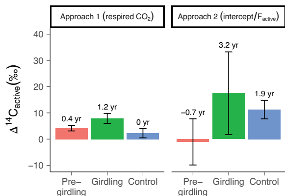
FIGURE 5 The \Delta^{14}\text{C} signatures and mean age estimations of the active C pool according to two approaches; approach 1 assumes \Delta^{14}\text{C}_{\text{active}} equals to the \Delta^{14}\text{C} signature of respired \text{CO}_2 ( \Delta^{14}\text{C}_{\text{resp}} ); approach 2 is based on the intercept and slope estimates of the fitted linear line between the \Delta^{14}\text{C} signatures of the extracted water-soluble C ( \Delta^{14}\text{C}_{\text{ws}} ) and \alpha -cellulose C ( \Delta^{14}\text{C}_{\text{cell}} ). According to this approach the fraction of the active C pool F_{\text{active}} = 1 - \text{slope} . Roots collected before girdling (Pre-girdling), ~3 months after girdling (Girdling) and ~3 months after girdling but in un-girdled trees (Control). One set of roots was used for respiration incubations ( n = 12 ) and second set was used for the C extractions ( n = 23 , 12, 11, respectively). Error bars of approach 1 is the standard errors of the \Delta^{14}\text{C}_{\text{resp}} results, and of approach 2 are the cumulative standard errors of the slope and intercept estimates [Colour figure can be viewed at wileyonlinelibrary.com ]
