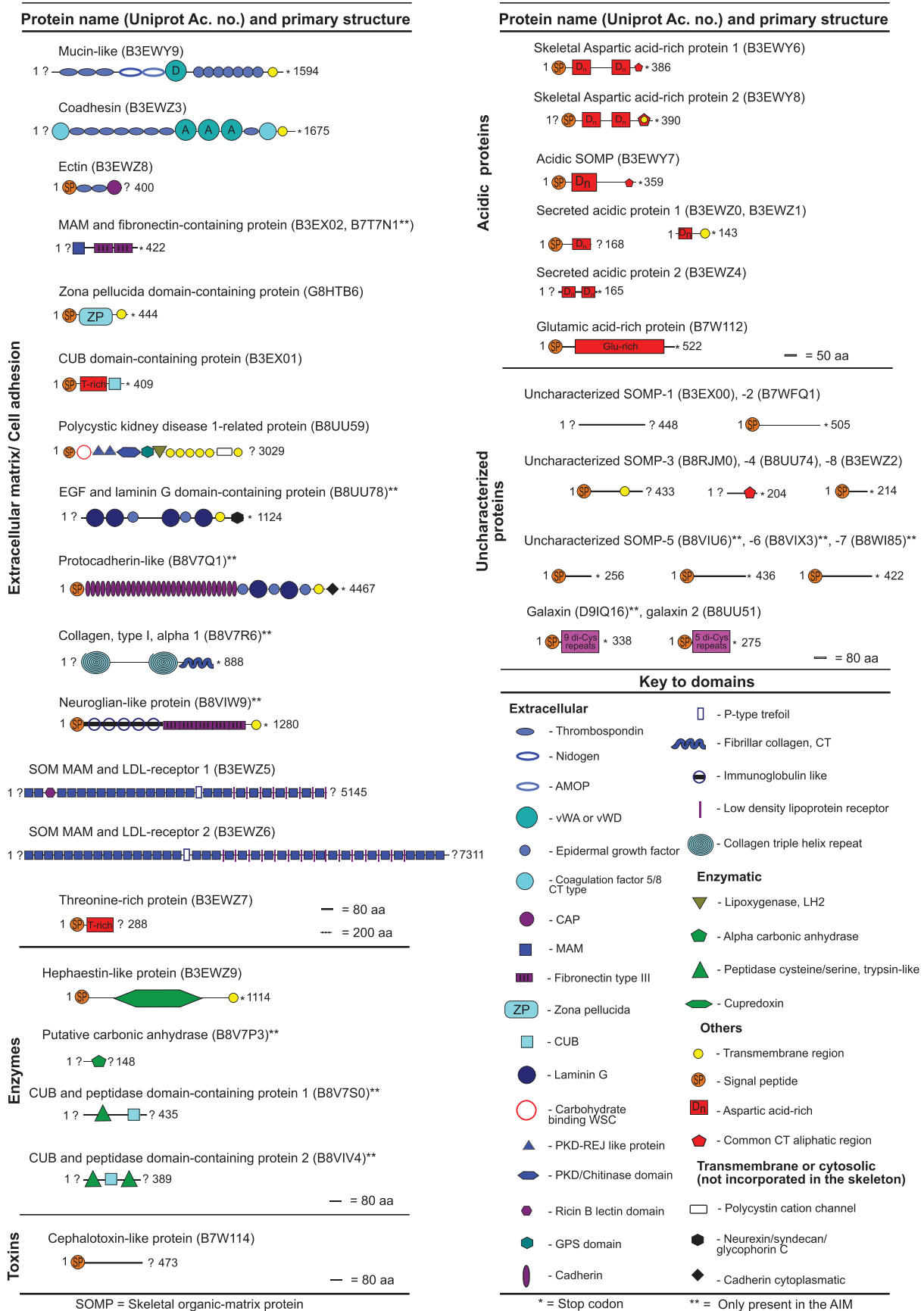
FIG. 3. List of SOMPs identified by proteomics in the acid soluble and insoluble matrices extracted from Acropora millepora skeleton. Proteins were named according to the characterization of their primary structure.
