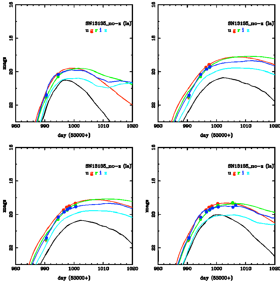
Figure 6. Light curves of SN2006fz (the same SN as shown in Figure 5) and fits to the best-fit SN Ia models after 2, 4, 6, and 8 epochs of detections without a galaxy photometric redshift prior. Search photometry from gri are shown. Model light curves in u and z are shown as well.
