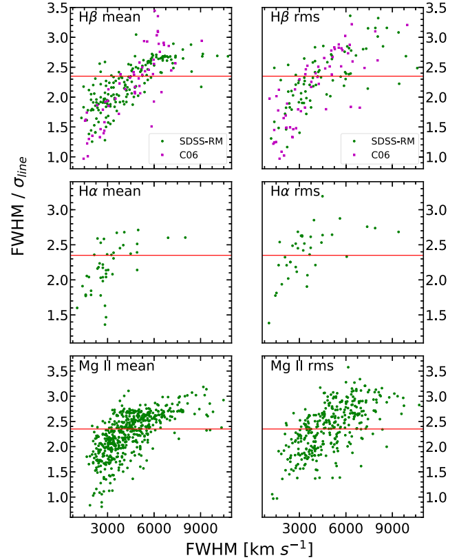
Figure 6. Line shape parameter \text{FWHM}/\sigma_{\text{line}} as a function of FWHM of mean spectra (left) and rms spectra (right). The results for \text{H}\beta , \text{H}\alpha , and \text{Mg II} are shown from top to bottom, respectively. The red horizontal line corresponds to the Gaussian profile with \text{FWHM}/\sigma_{\text{line}} = 2.35 .
