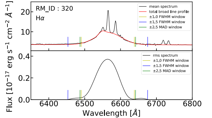
Figure 9. Illustration of the three different choices of window size. The black solid lines in the top and bottom panels represent the mean and rms spectra, respectively. The red line is the total broad-line profile in the mean spectrum used to calculate different line widths. The yellow, blue, and green vertical lines represent 1.0 \times \text{FWHM} window, 1.5 \times \text{FWHM} window, and 2.5 \times \text{MAD} window, respectively.
