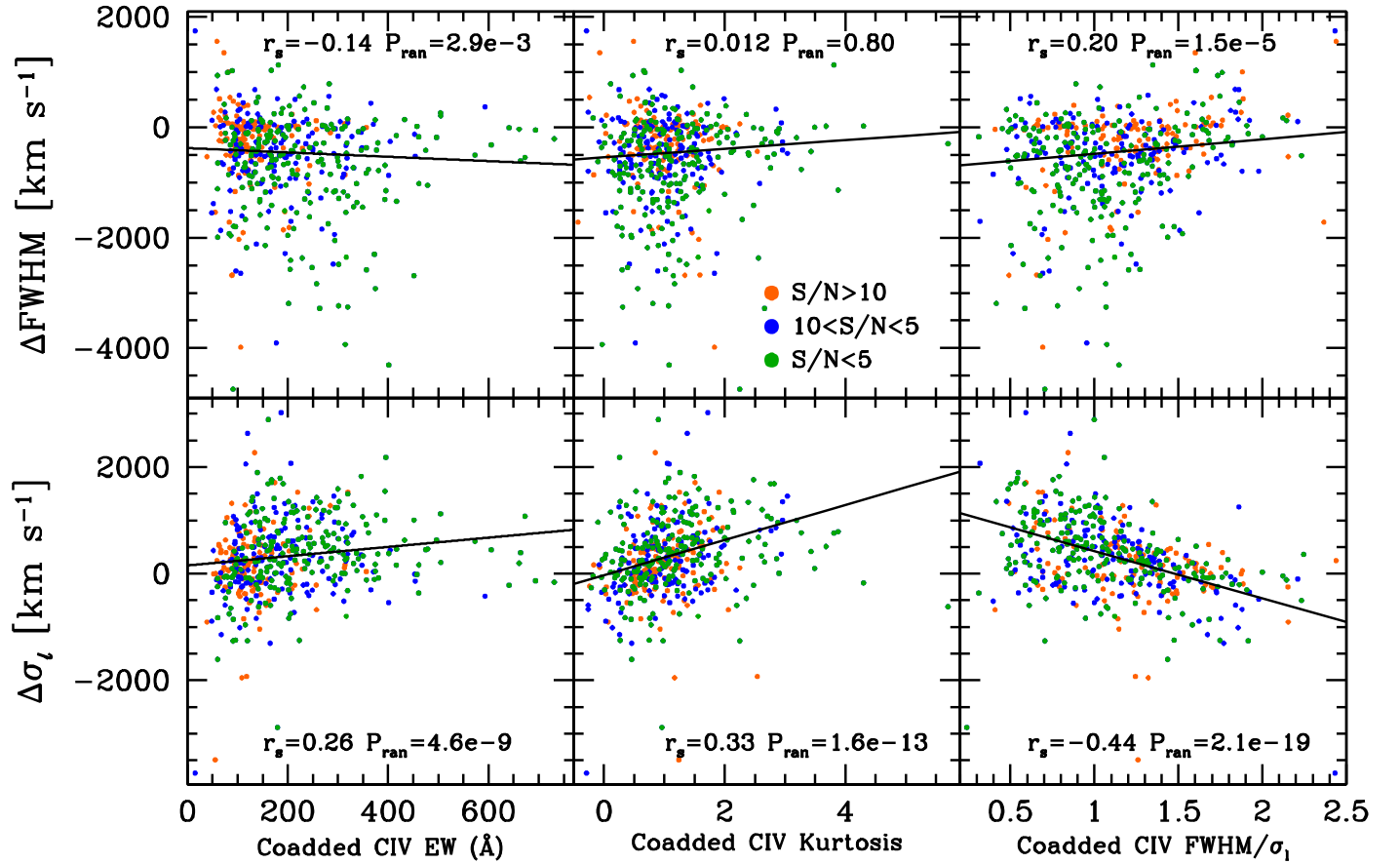
Figure 10. C IV line-width differences as a function of other C IV emission line properties. The top (bottom) panels show results based on the FWHM (line dispersion, \sigma_l ). The left, middle, and right panels show the dependence of the difference on the C IV EW, kurtosis, and shape (FWHM/ \sigma_l ), respectively. The points are color-coded by the varying data quality of each subsample: S/N > 10 (orange), 10 < S/N < 5 (blue), and S/N < 5 (green). The solid black lines show the best-fit linear regression fit. The Spearman rank correlation coefficient, r_s , and the probability that a correlation is found by chance, P_{\text{ran}} , are given in each panel.
