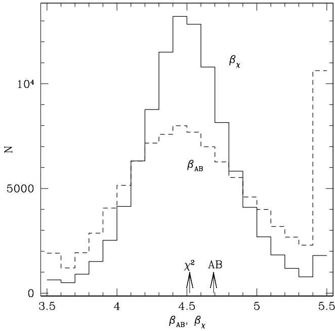
FIG. 1.—Distribution of the estimators \beta_x (eq. [3]; solid line) and \beta_{AB} (eq. [5]; dashed line) for 100,000 Monte Carlo simulations of a sample with \beta = 4.5 that resembles the actual sample FM1 (12 galaxies, distributed as a Gaussian with standard deviation 0.20 in x , and Gaussian measurement errors with standard deviations \epsilon_x = 0.06 , \epsilon_y = 0.18 ). Values greater than 5.5 or less than 3.3 are plotted in the outermost bins of the histogram. The sample means are marked by arrows.
