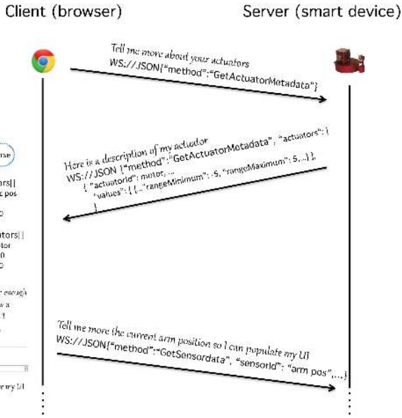
Fig. 5. The web client asks the Smart Device about the available actuators.
