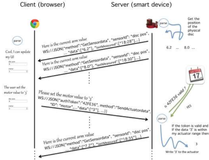
Fig. 6. The Smart Device pushes the measured values to the client. It also receives and validates the actuator value prior to apply it to the motor.
