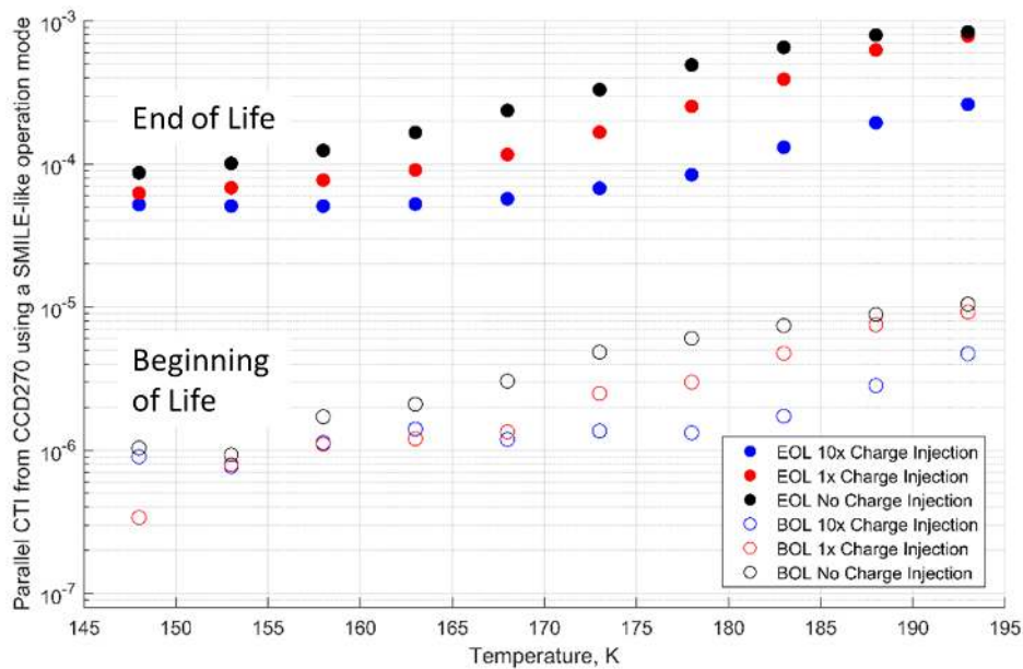
Figure 6. Parallel CTI performance of a PLATO CCD270 operated in SMILE-like conditions (6x6 binning and timing). The parallel CTI is defined as the proportion of signal lost per native pixel transfer.
