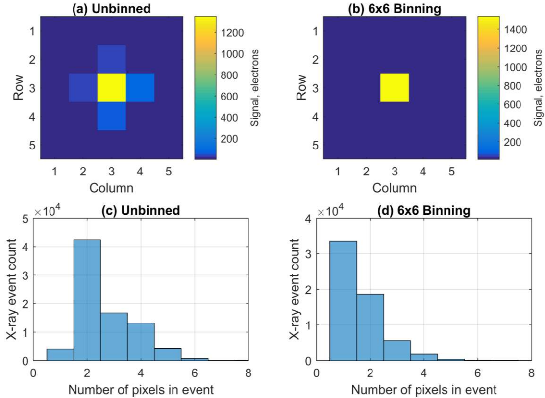
Figure 5. 6x6 pixel binning confines the majority of X-ray events to one or two pixels. The average X-ray event observed in the unirradiated region of interest at 148 K is seen to have signal split into neighbouring pixels when not binned (a), but confined to a single pixel when binned (b). The number of pixels above a threshold ( 4.5\times the background noise) for each of the binning modes also shows the shift of multi-pixel events when not binning (c) to primarily 1 or 2 pixel events when binning is applied (d).
