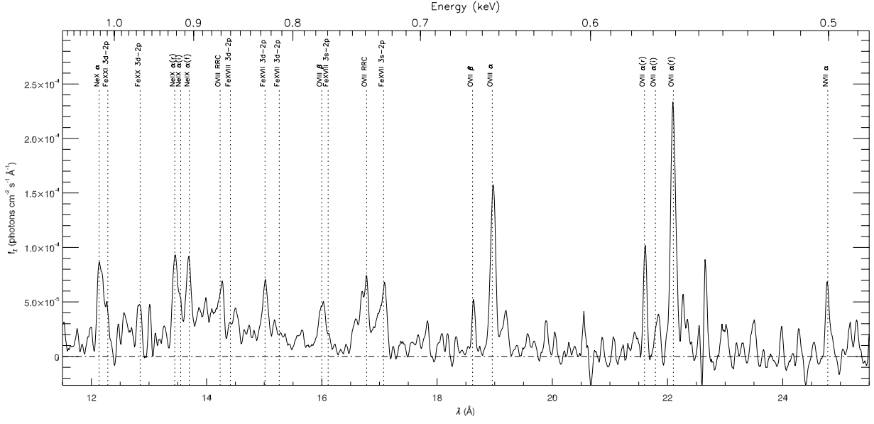
Fig. 4. Mrk 3: XMM-Newton 190 ks combined RGS spectrum, plotted in the rest frame of the source (12–25 Å). The strongest emission features are labelled.
