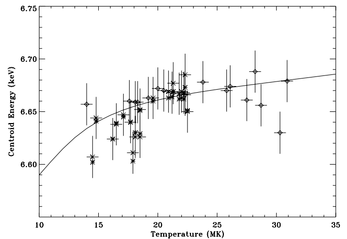
FIG. 4.—Centroid energy of the Fe line feature, observed with a spectrometer like RHESSI having a resolution with FWHM 0.8 keV, compared with observed points from the SMM Bent Crystal Spectrometer (asterisks) and the Yohkoh Bragg Crystal Spectrometer (diamonds) for large flares on 1980 July 1 and 1991 December 16, respectively.
