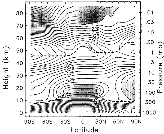
January temperature
