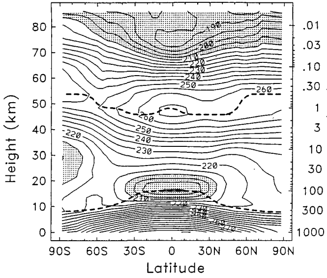
April temperature
