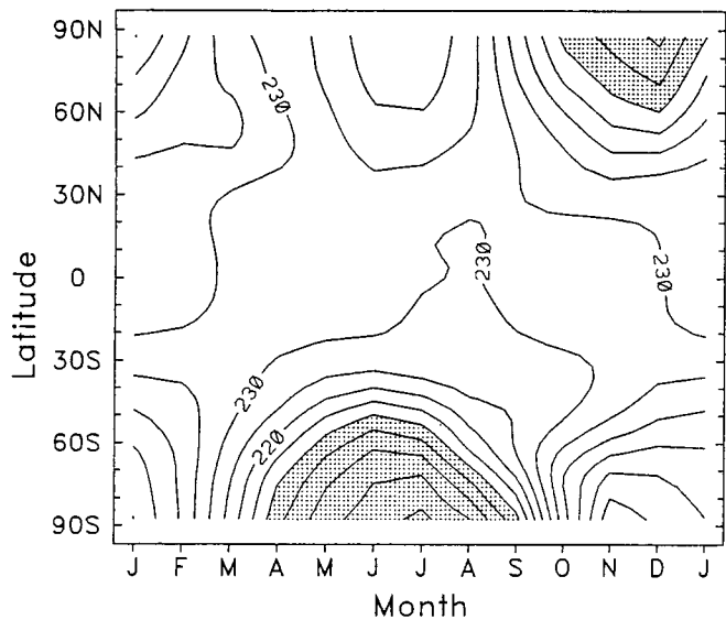
Temperature 10hPa
