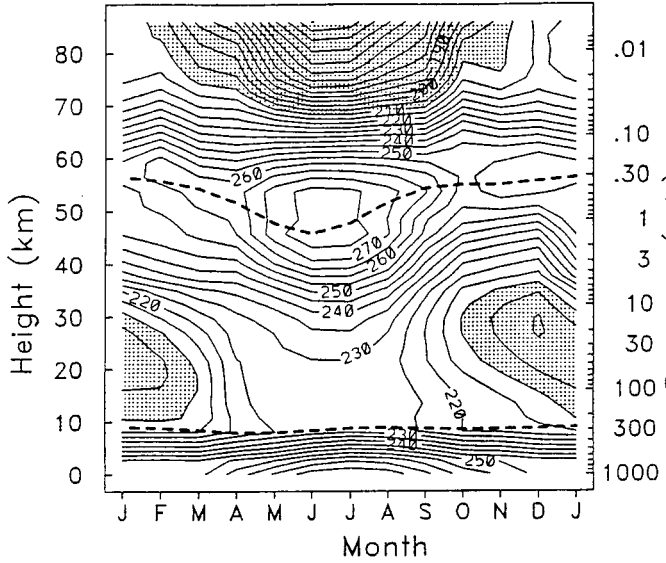
Temperature 80N
