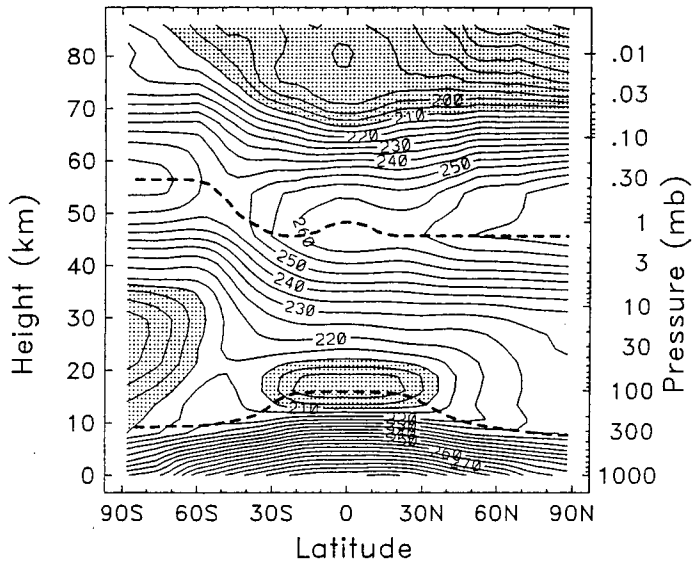
May temperature
