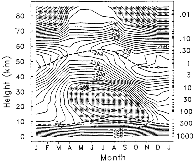
Temperature 80S
