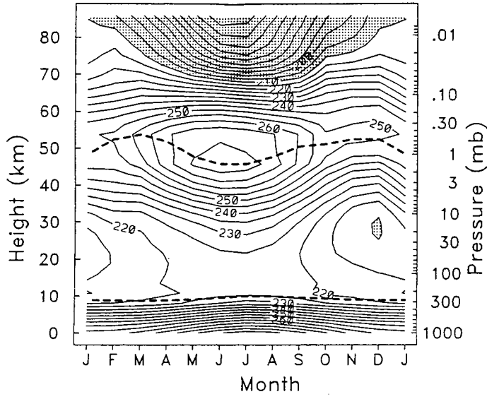
Temperature 60N
