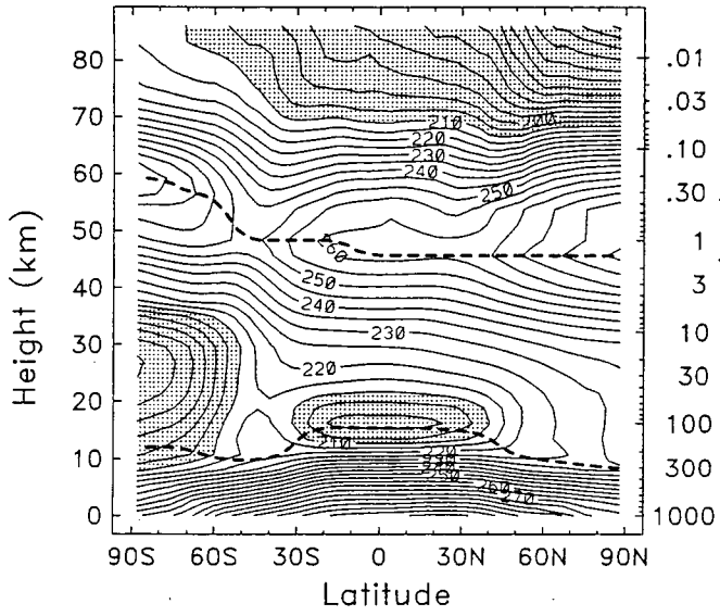
July temperature
