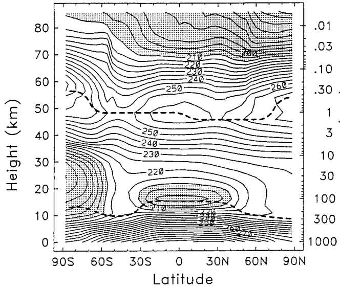
August temperature
