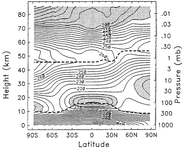
November temperature
