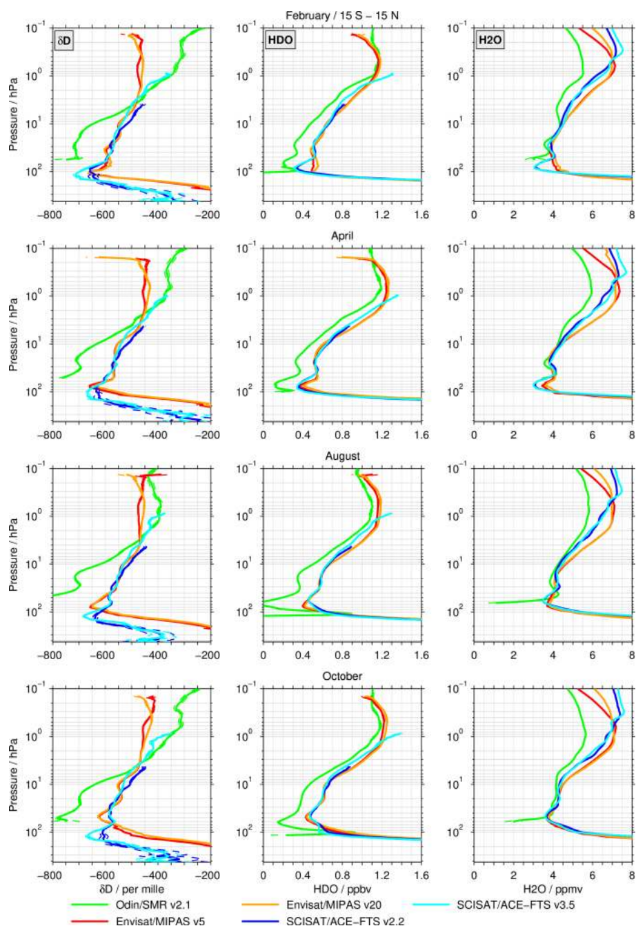
Figure 10. Tropical mean ( 15^{\circ}\text{S} – 15^{\circ}\text{N} ) profiles for \delta D (left column panels), HDO (middle column), and H 2 O (right column panels) for February, April, August, and October given in different rows.
