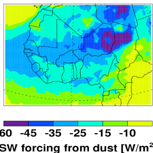
Fig. 12. Clear-sky surface SW dust radiative forcing at 12:00 UTC over North Africa for the simulation period estimated from the WRF-Chem simulations in the Sect1-G case. The SW dust radiative forcing is estimated by subtracting the result from the simulation without dust emissions from that from the simulation with dust emissions.
