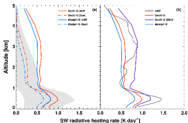
Fig. 11. (a) SW aerosol (solid line) and dust (dot dash line) heating profiles from the WRF-Chem simulations in different cases at 08:00–12:00 UTC for the DABEX period at the Niamey airport. The gray area represents the variation of Sect1-G simulated SW dust heating rate due to the uncertainty of n_i (imaginary part of refractive index) of mineral dust; (b) SW aerosol heating profiles from the calculations based on the AMF retrievals and the WRF-Chem simulations in different cases at 08:00–12:00 UTC for the DABEX period at the Niamey airport.
