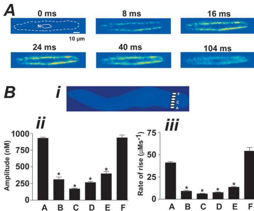
Fig. 1. Spatially heterogeneous Ca 2+ transients during EC-coupling in atrial myocytes. (A) A representative myocyte displaying Ca 2+ transients at a series of time points (in milliseconds) after depolarisation of the cells. Transients were restricted to the junctional periphery. The solid white line denotes the position of the nucleus (N) and the dotted line indicates the cell periphery. The times noted on top of the images indicate the instances at which the images were taken relative to cell depolarisation. (B) A quantitative analysis of the propagation of electrically evoked Ca 2+ signals in an atrial myocyte. The cell is depicted in i and the six regions from which the Ca 2+ signal was sampled are indicated running transversely across the cell (denoted 'A' to 'F'). The average amplitude (ii) and rate of rise of the calcium signal (iii) in each region were calculated from six successive depolarisations, and are shown as mean±s.e.m. *Significantly different ( P <0.05) from the response in region A. Please note that before each experimental recording, cells were paced until they had reached a steady-state condition.
