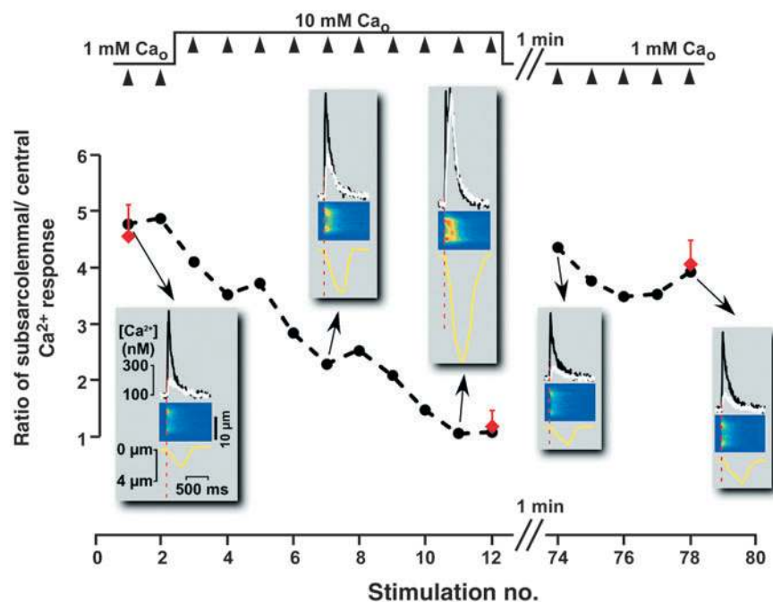
Fig. 2. Increased Ca 2+ influx enhances the response of the central non-junctional RyRs. The top portion of the figure depicts the experimental protocol. The arrowheads indicate the points at which cells were depolarised. The transformation in the spatial distribution of action potential-evoked Ca 2+ signals is shown by the change in the ratio of Ca 2+ signal amplitude in the subsarcolemmal space relative to central regions. The filled circles denote the response of the myocyte from which the inset traces were obtained, and the red diamonds show the mean±s.e.m. from six cells (two each from three rats). The inset panels illustrate the time course and amplitude of the Ca 2+ signal at subsarcolemmal (black trace) and central (white traces) regions. A pseudo-linescan is shown beneath the traces to illustrate the spatial properties of the recorded Ca 2+ signals. The yellow trace under the pseudo-linescan image indicates the extent of cellular contraction and the vertical dashed red line, the onset of depolarisation.
